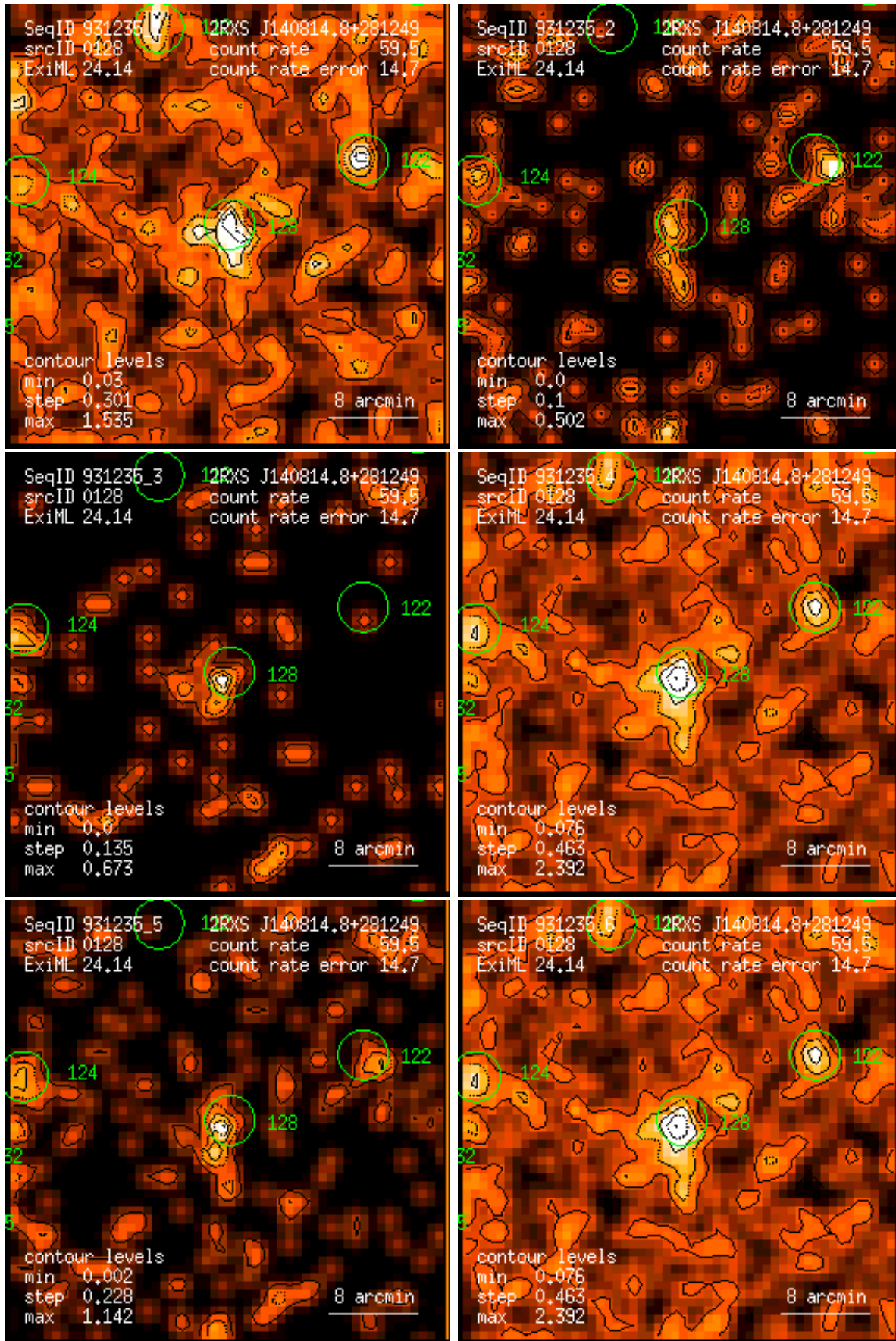
Figure 128: RASS 931235: detection 0128: band rate images, Gaussian filter: (1) PSPC channels 11 – 41, (2) 52 – 90, (3) 91 – 201, (4) 11 – 235, (5) 52 – 201, (6) 11 – 201. Broad band rates in counts/ks. Band rate contour levels in counts/ks/arcmin 2 .
