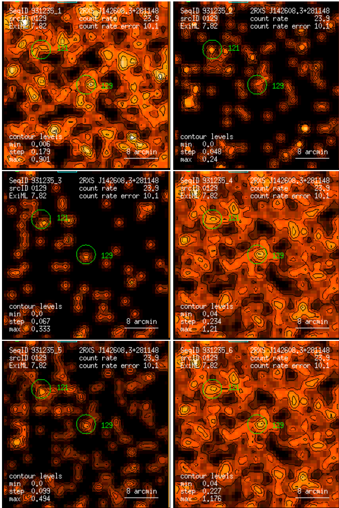
Figure 129: RASS 931235: detection 0129: band rate images, Gaussian filter: (1) PSPC channels 11 – 41, (2) 52 – 90, (3) 91 – 201, (4) 11 – 235, (5) 52 – 201, (6) 11 – 201. Broad band rates in counts/ks. Band rate contour levels in counts/ks/arcmin 2 .
