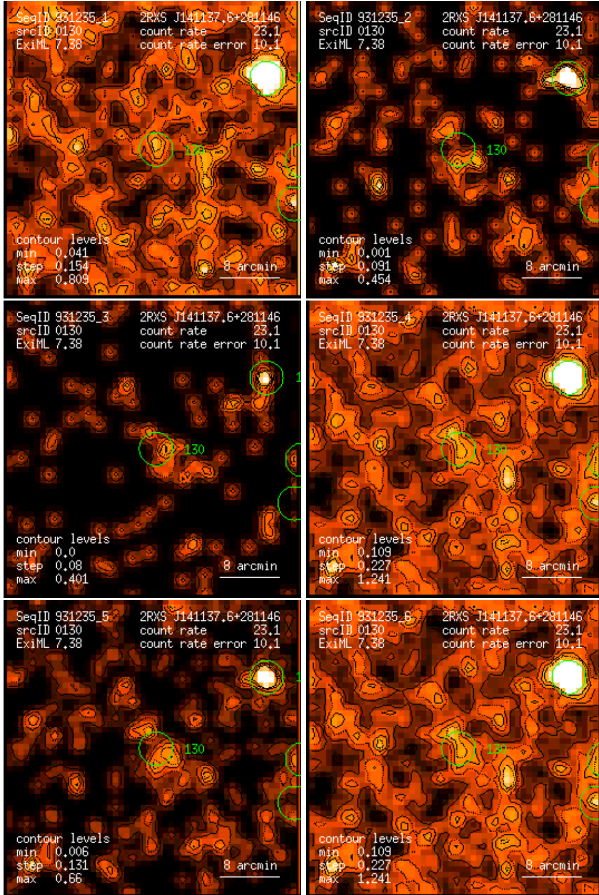
Figure 130: RASS 931235: detection 0130: band rate images, Gaussian filter: (1) PSPC channels 11 – 41, (2) 52 – 90, (3) 91 – 201, (4) 11 – 235, (5) 52 – 201, (6) 11 – 201. Broad band rates in counts/ks. Band rate contour levels in counts/ks/arcmin 2 .
