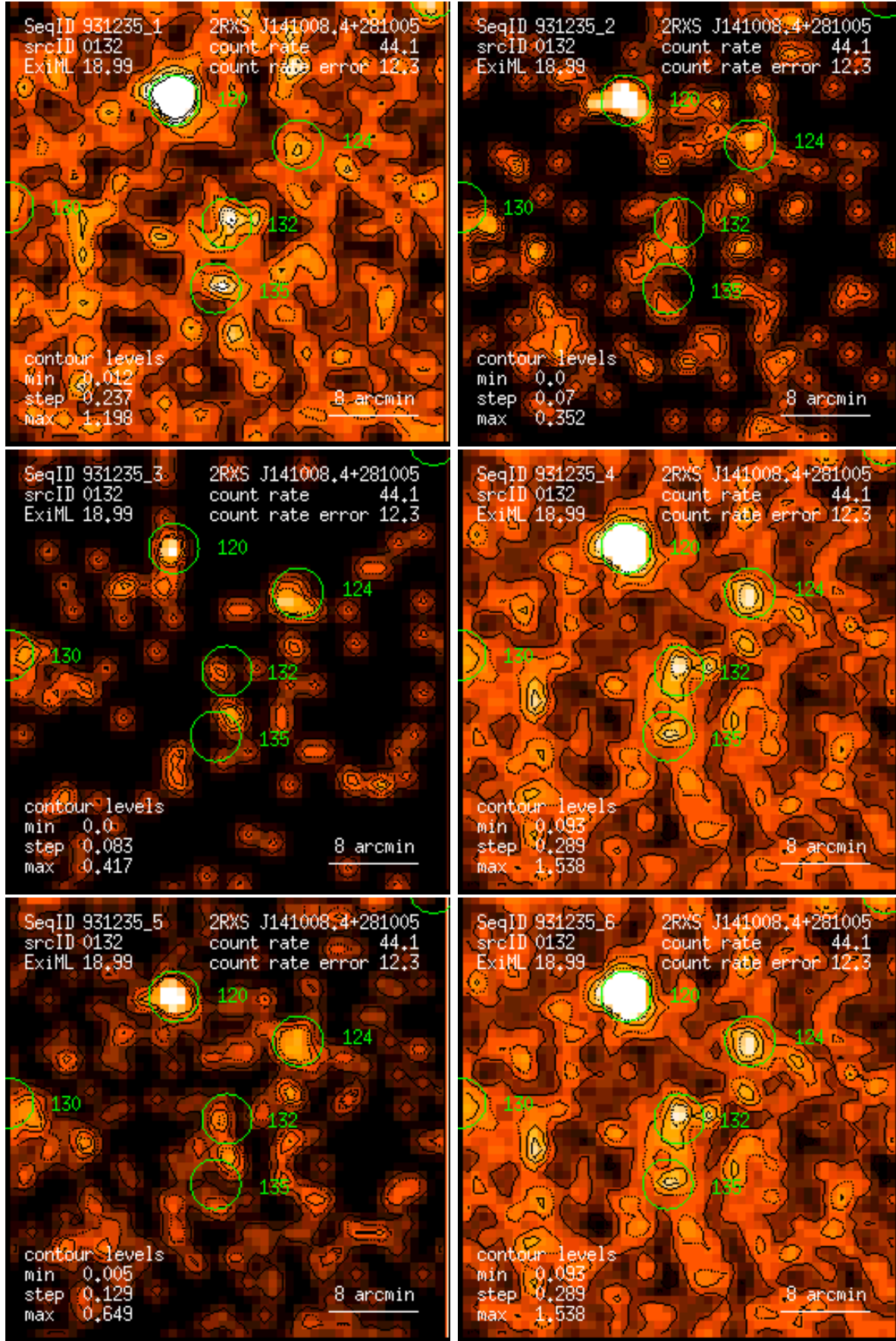
Figure 132: RASS 931235: detection 0132: band rate images, Gaussian filter: (1) PSPC channels 11 – 41, (2) 52 – 90, (3) 91 – 201, (4) 11 – 235, (5) 52 – 201, (6) 11 – 201. Broad band rates in counts/ks. Band rate contour levels in counts/ks/arcmin 2 .
