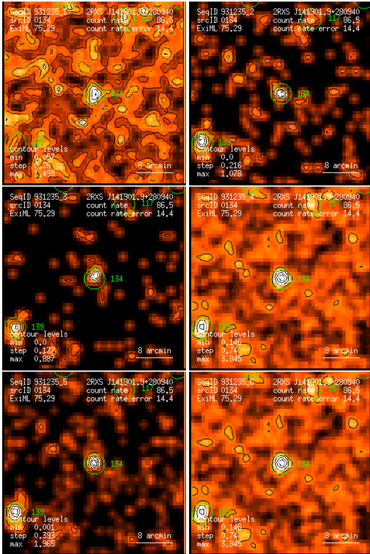
Figure 134: RASS 931235: detection 0134: band rate images, Gaussian filter: (1) PSPC channels 11 – 41, (2) 52 – 90, (3) 91 – 201, (4) 11 – 235, (5) 52 – 201, (6) 11 – 201. Broad band rates in counts/ks. Band rate contour levels in counts/ks/arcmin 2 .
