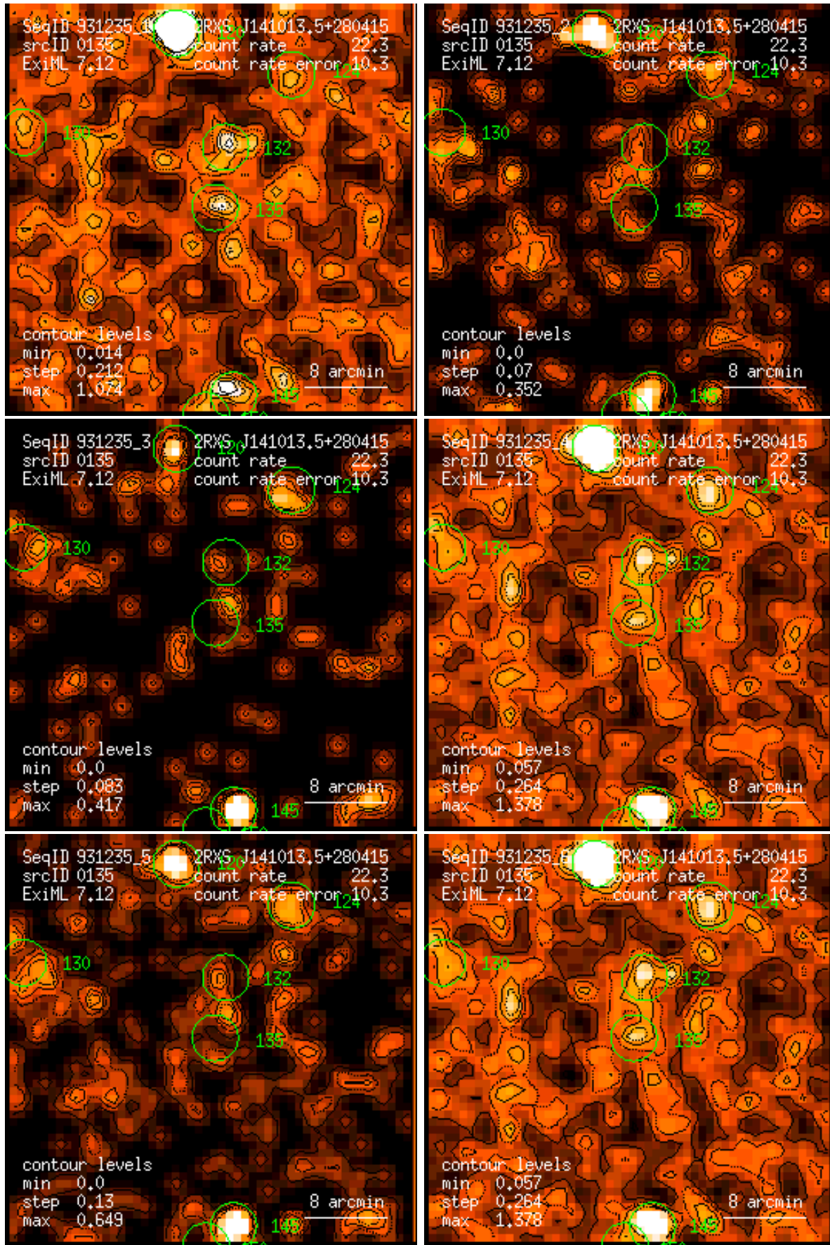
Figure 135: RASS 931235: detection 0135: band rate images, Gaussian filter: (1) PSPC channels 11 – 41, (2) 52 – 90, (3) 91 – 201, (4) 11 – 235, (5) 52 – 201, (6) 11 – 201. Broad band rates in counts/ks. Band rate contour levels in counts/ks/arcmin 2 .
