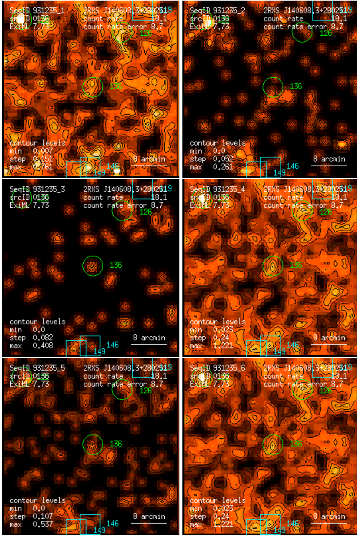
Figure 136: RASS 931235: detection 0136: band rate images, Gaussian filter: (1) PSPC channels 11 – 41, (2) 52 – 90, (3) 91 – 201, (4) 11 – 235, (5) 52 – 201, (6) 11 – 201. Broad band rates in counts/ks. Band rate contour levels in counts/ks/arcmin 2 .
