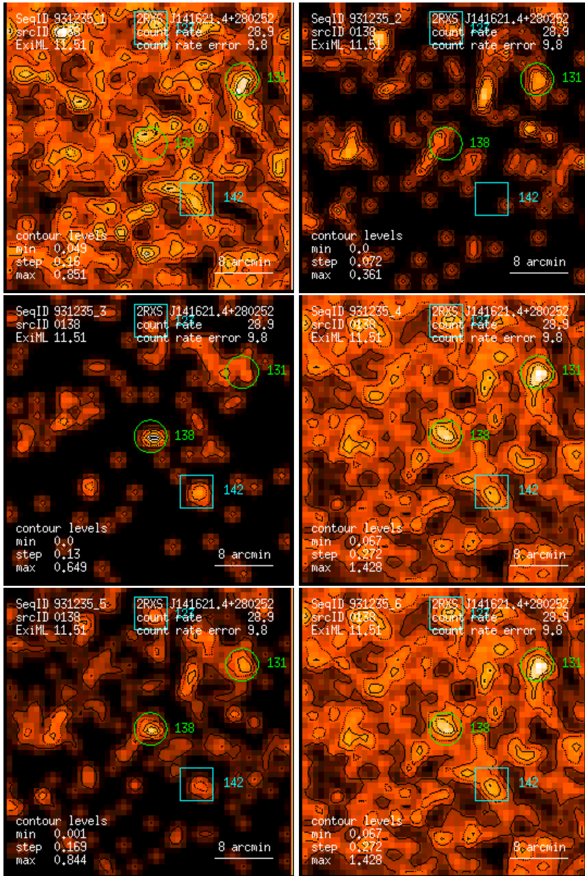
Figure 138: RASS 931235: detection 0138: band rate images, Gaussian filter: (1) PSPC channels 11 – 41, (2) 52 – 90, (3) 91 – 201, (4) 11 – 235, (5) 52 – 201, (6) 11 – 201. Broad band rates in counts/ks. Band rate contour levels in counts/ks/arcmin 2 .
