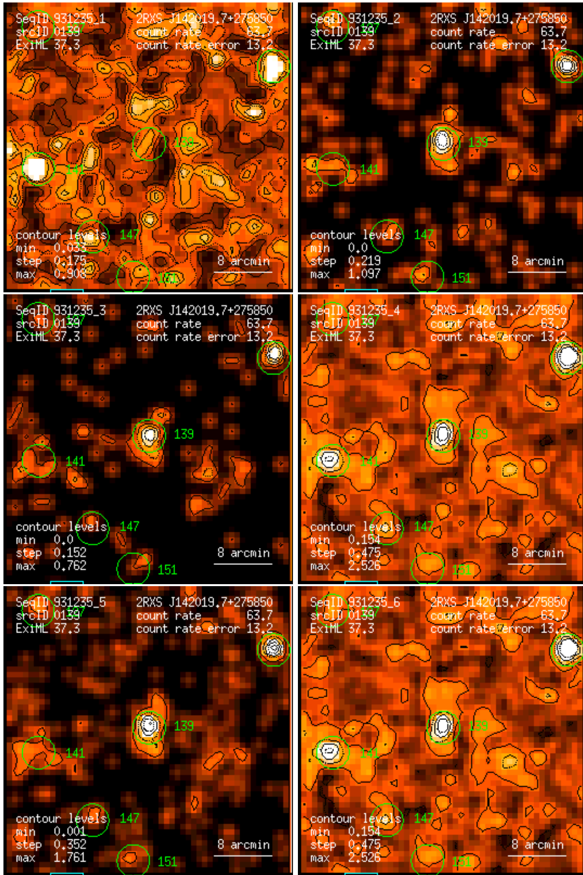
Figure 139: RASS 931235: detection 0139: band rate images, Gaussian filter: (1) PSPC channels 11 – 41, (2) 52 – 90, (3) 91 – 201, (4) 11 – 235, (5) 52 – 201, (6) 11 – 201. Broad band rates in counts/ks. Band rate contour levels in counts/ks/arcmin 2 .
