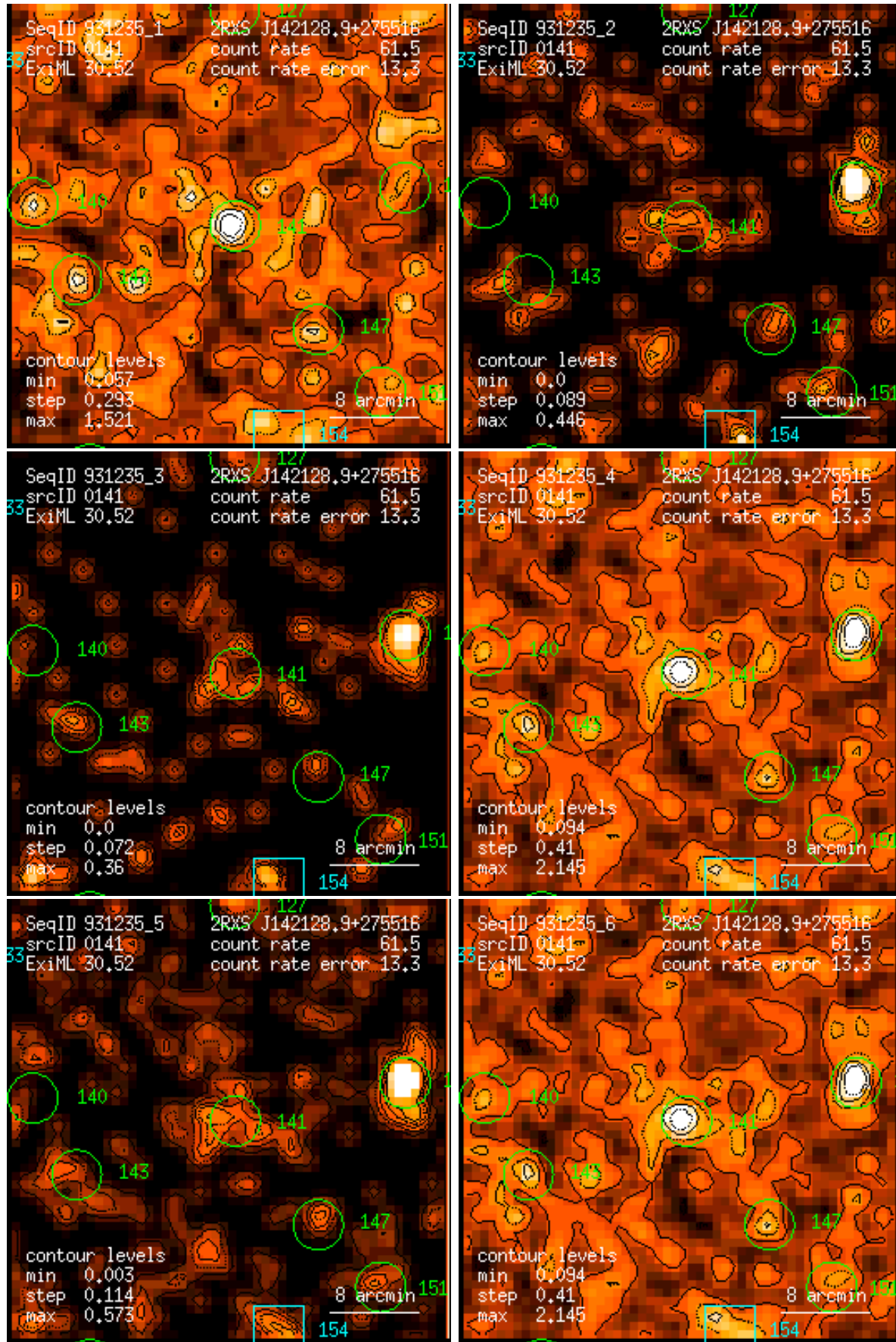
Figure 141: RASS 931235: detection 0141: band rate images, Gaussian filter: (1) PSPC channels 11 – 41, (2) 52 – 90, (3) 91 – 201, (4) 11 – 235, (5) 52 – 201, (6) 11 – 201. Broad band rates in counts/ks. Band rate contour levels in counts/ks/arcmin 2 .
