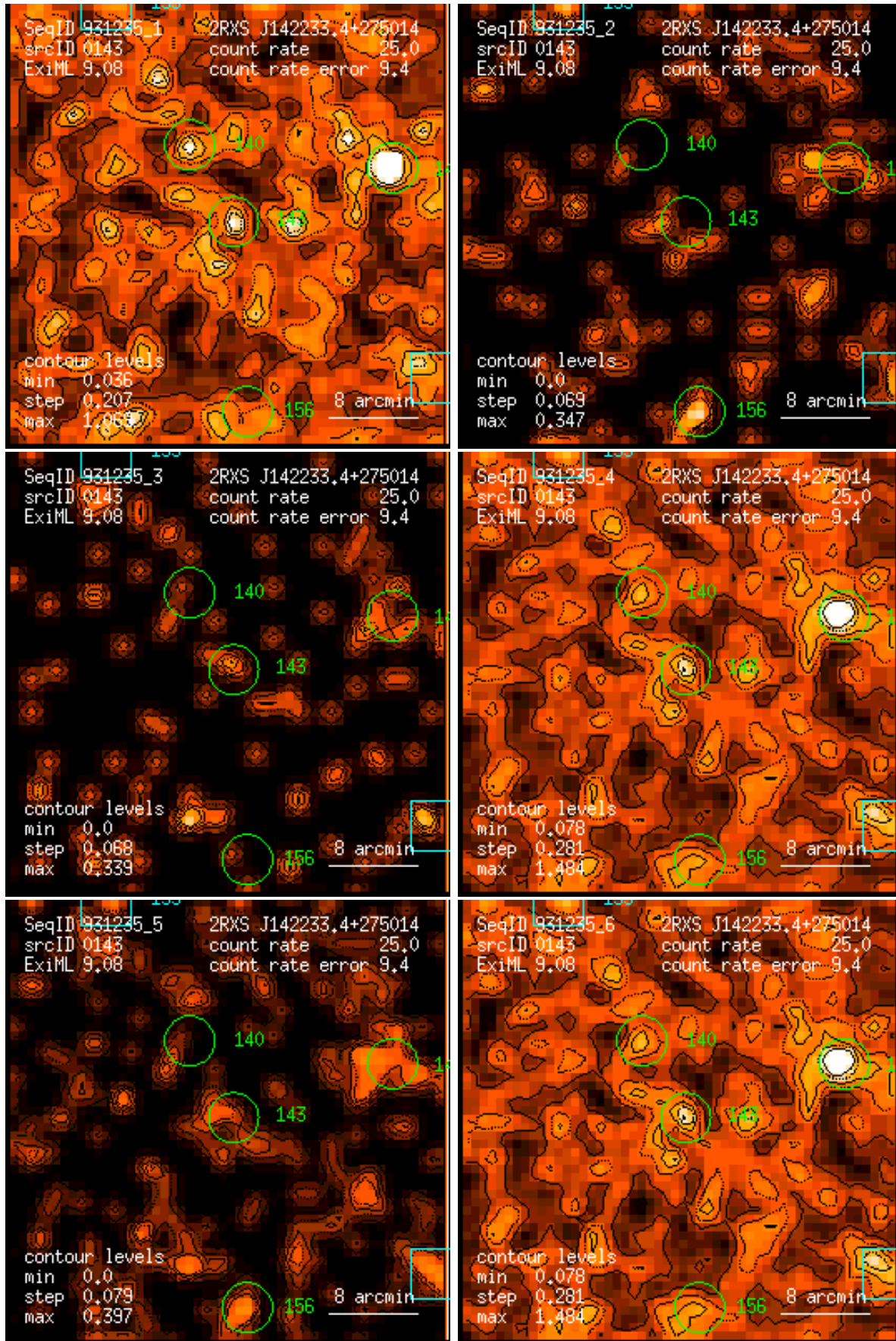
Figure 143: RASS 931235: detection 0143: band rate images, Gaussian filter: (1) PSPC channels 11 – 41, (2) 52 – 90, (3) 91 – 201, (4) 11 – 235, (5) 52 – 201, (6) 11 – 201. Broad band rates in counts/ks. Band rate contour levels in counts/ks/arcmin 2 .
