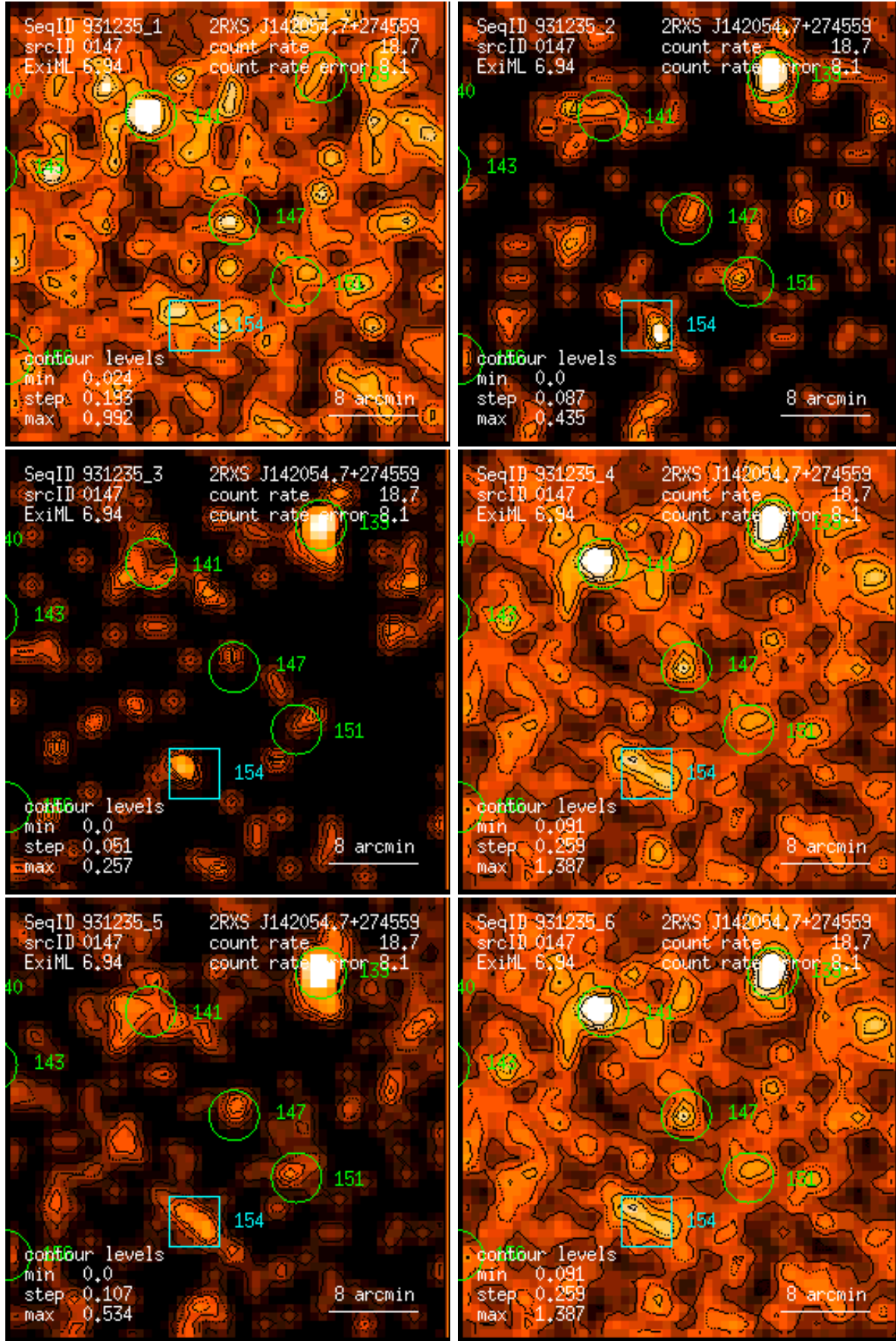
Figure 147: RASS 931235: detection 0147: band rate images, Gaussian filter: (1) PSPC channels 11 – 41, (2) 52 – 90, (3) 91 – 201, (4) 11 – 235, (5) 52 – 201, (6) 11 – 201. Broad band rates in counts/ks. Band rate contour levels in counts/ks/arcmin 2 .
