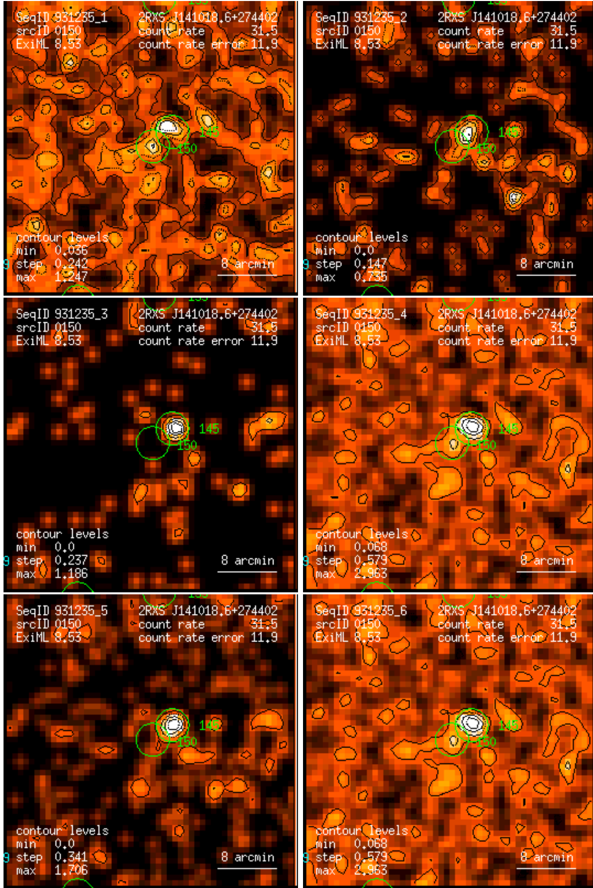
Figure 150: RASS 931235: detection 0150: band rate images, Gaussian filter: (1) PSPC channels 11 – 41, (2) 52 – 90, (3) 91 – 201, (4) 11 – 235, (5) 52 – 201, (6) 11 – 201. Broad band rates in counts/ks. Band rate contour levels in counts/ks/arcmin 2 .
