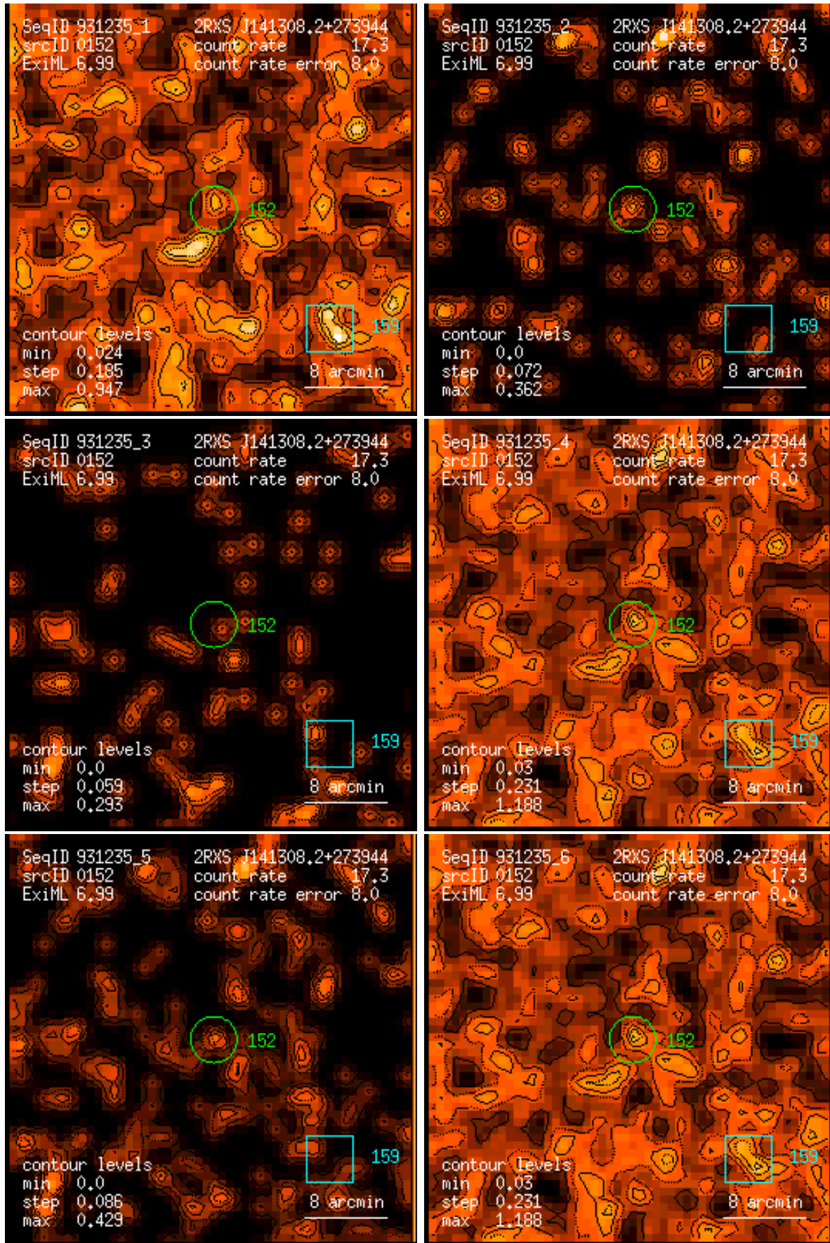
Figure 152: RASS 931235: detection 0152: band rate images, Gaussian filter: (1) PSPC channels 11 – 41, (2) 52 – 90, (3) 91 – 201, (4) 11 – 235, (5) 52 – 201, (6) 11 – 201. Broad band rates in counts/ks. Band rate contour levels in counts/ks/arcmin 2 .
