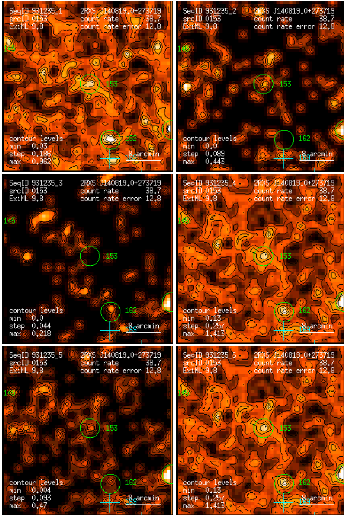
Figure 153: RASS 931235: detection 0153: band rate images, Gaussian filter: (1) PSPC channels 11 – 41, (2) 52 – 90, (3) 91 – 201, (4) 11 – 235, (5) 52 – 201, (6) 11 – 201. Broad band rates in counts/ks. Band rate contour levels in counts/ks/arcmin 2 .
