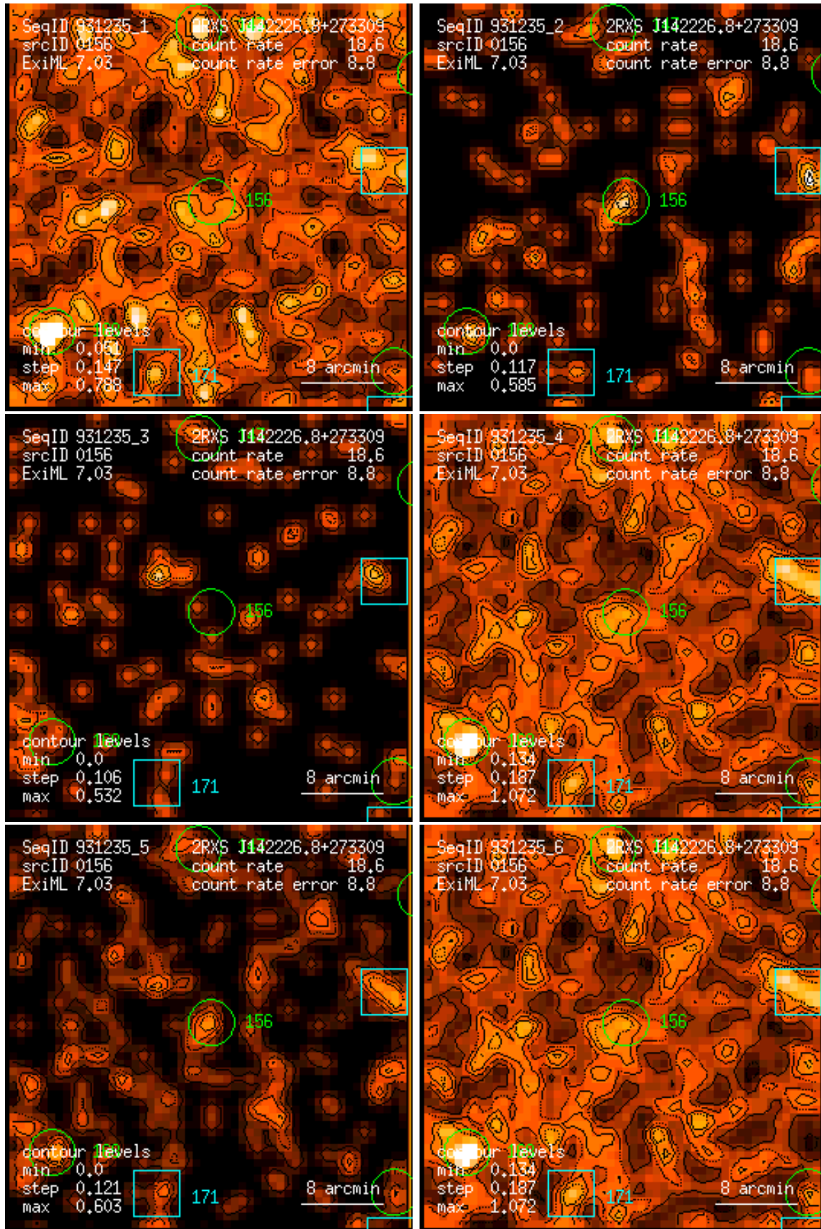
Figure 156: RASS 931235: detection 0156: band rate images, Gaussian filter: (1) PSPC channels 11 – 41, (2) 52 – 90, (3) 91 – 201, (4) 11 – 235, (5) 52 – 201, (6) 11 – 201. Broad band rates in counts/ks. Band rate contour levels in counts/ks/arcmin 2 .
