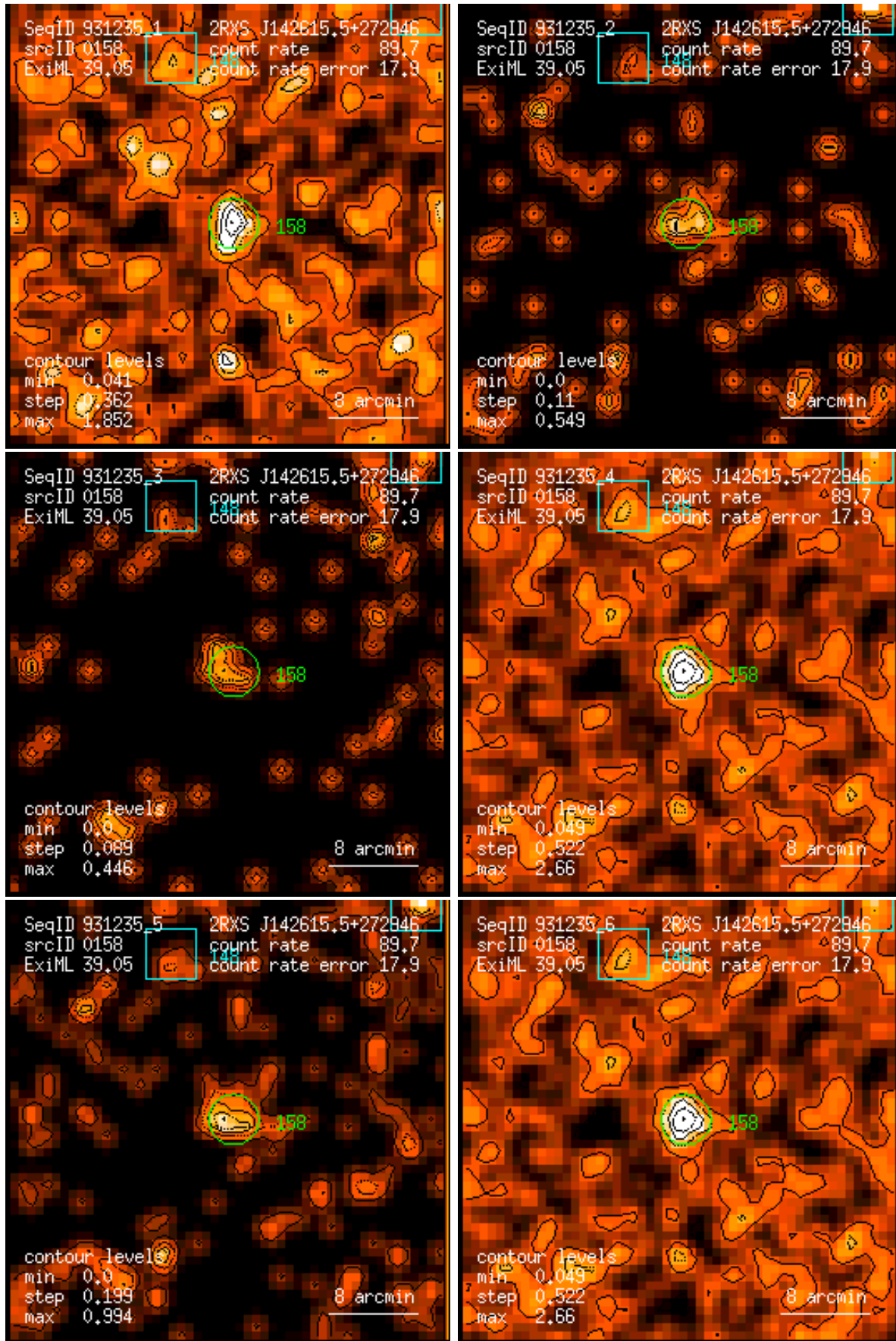
Figure 158: RASS 931235: detection 0158: band rate images, Gaussian filter: (1) PSPC channels 11 – 41, (2) 52 – 90, (3) 91 – 201, (4) 11 – 235, (5) 52 – 201, (6) 11 – 201. Broad band rates in counts/ks. Band rate contour levels in counts/ks/arcmin 2 .
