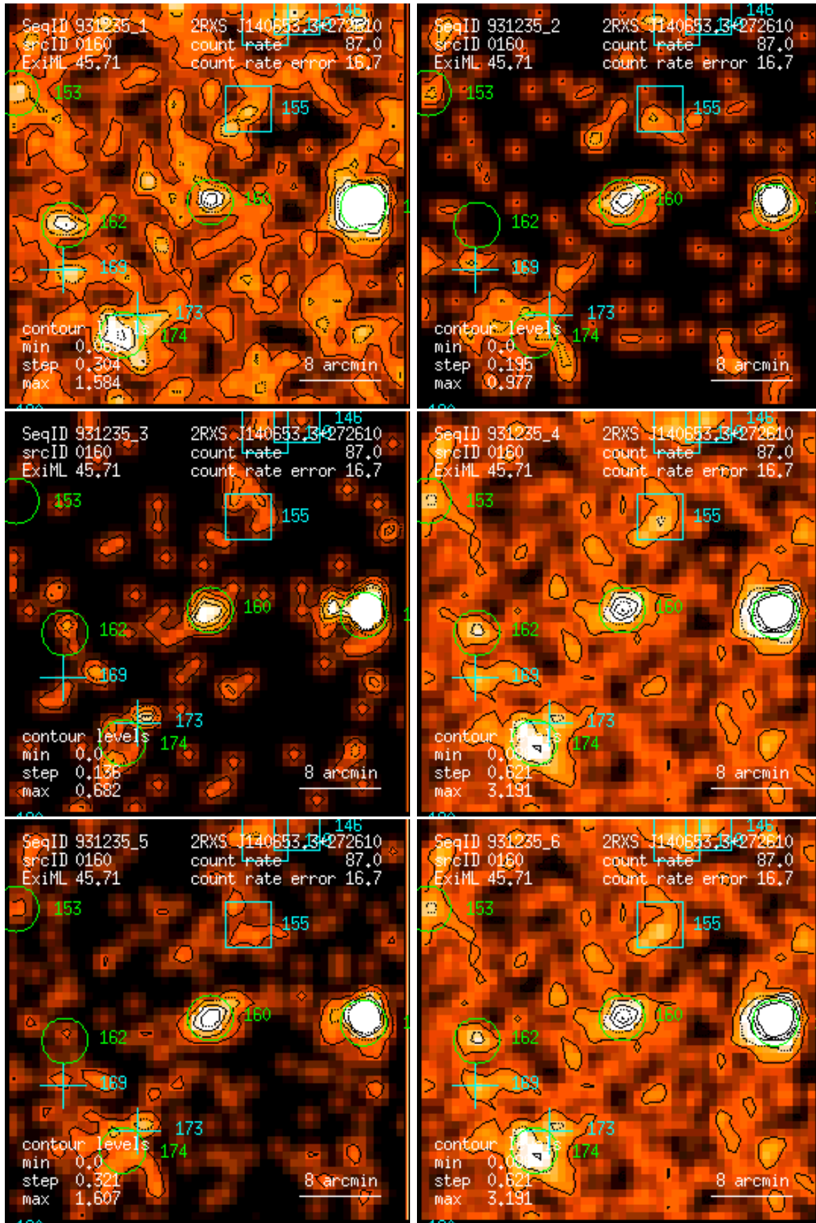
Figure 160: RASS 931235: detection 0160: band rate images, Gaussian filter: (1) PSPC channels 11 – 41, (2) 52 – 90, (3) 91 – 201, (4) 11 – 235, (5) 52 – 201, (6) 11 – 201. Broad band rates in counts/ks. Band rate contour levels in counts/ks/arcmin 2 .
