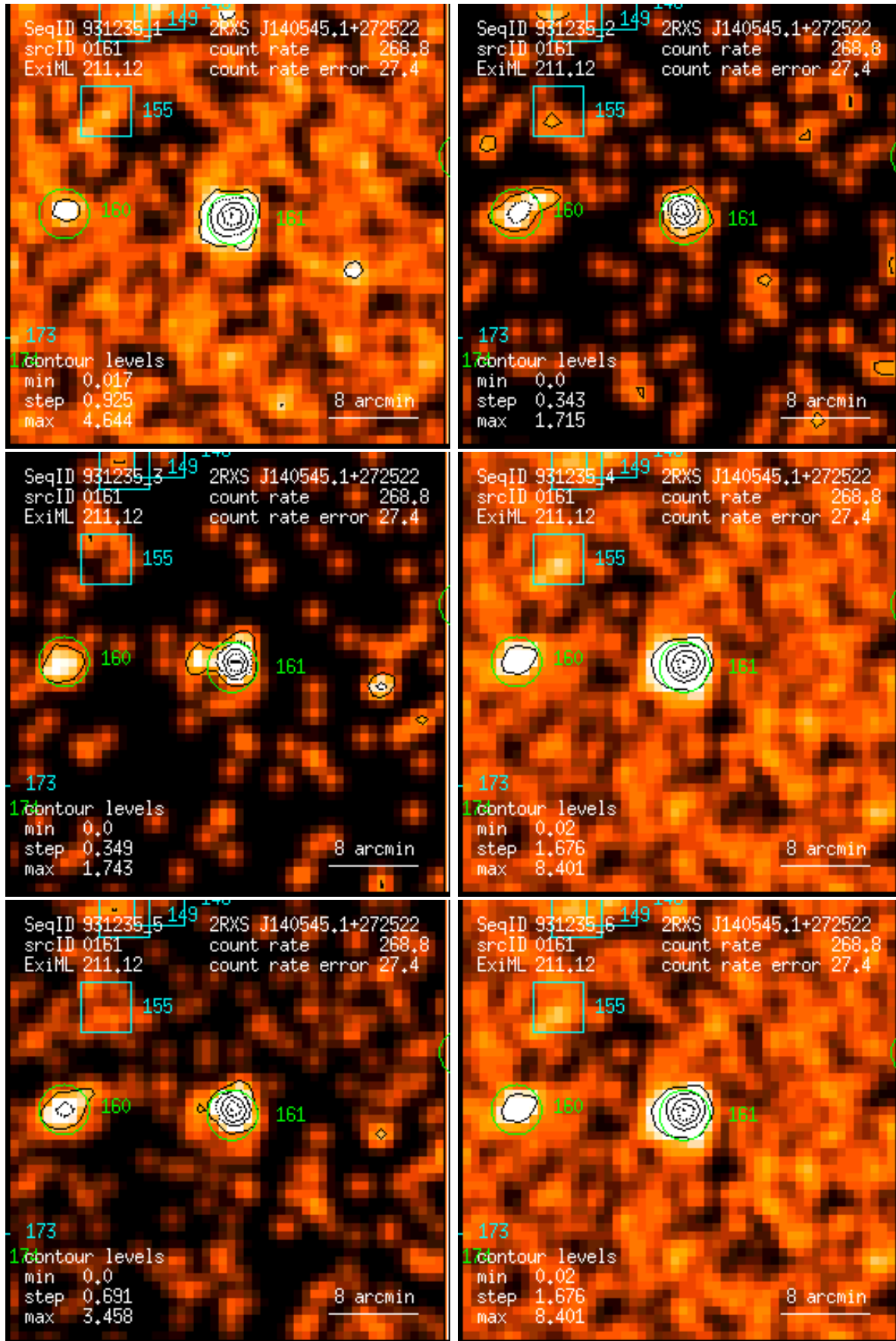
Figure 161: RASS 931235: detection 0161: band rate images, Gaussian filter: (1) PSPC channels 11 – 41, (2) 52 – 90, (3) 91 – 201, (4) 11 – 235, (5) 52 – 201, (6) 11 – 201. Broad band rates in counts/ks. Band rate contour levels in counts/ks/arcmin 2 .
