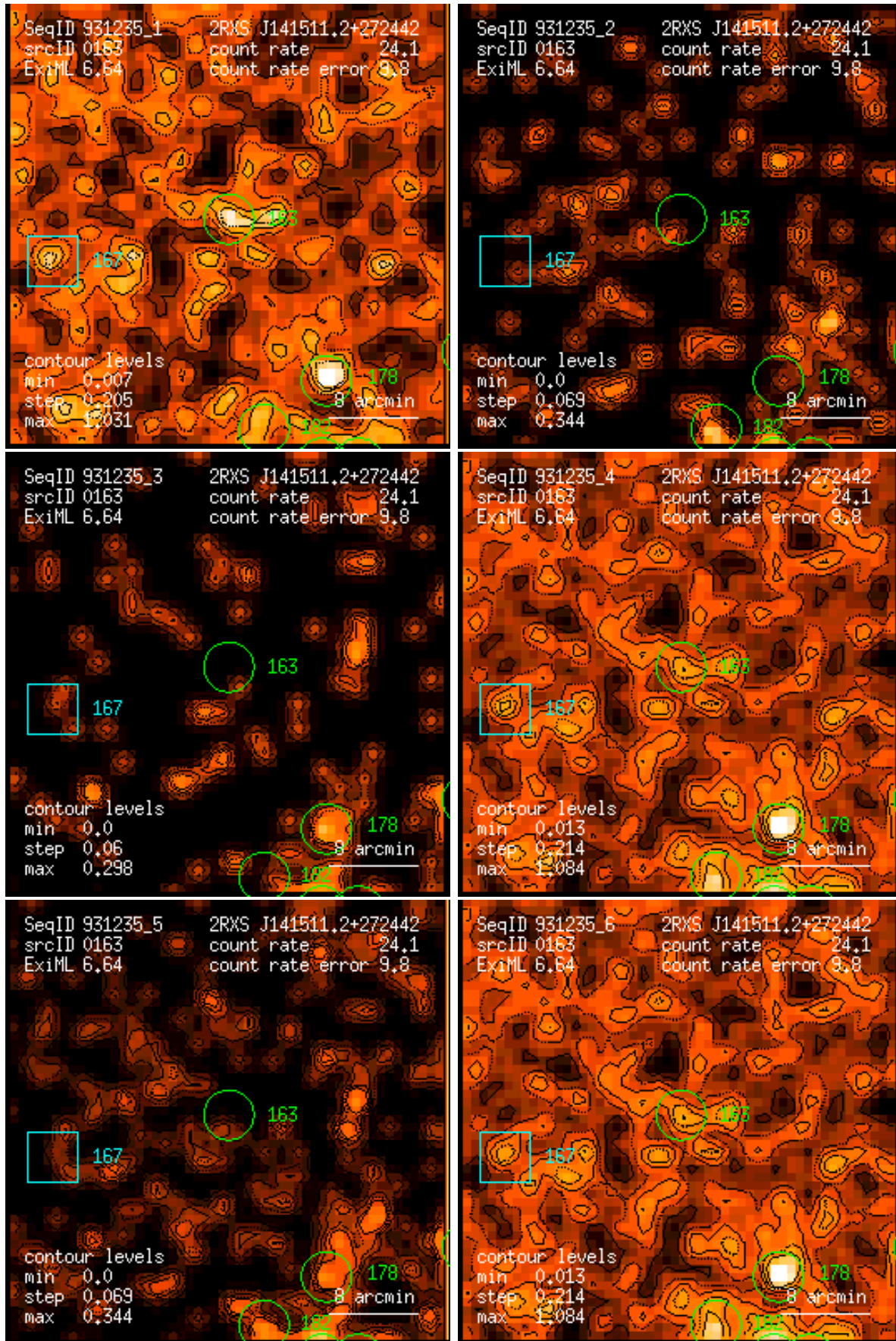
Figure 163: RASS 931235: detection 0163: band rate images, Gaussian filter: (1) PSPC channels 11 – 41, (2) 52 – 90, (3) 91 – 201, (4) 11 – 235, (5) 52 – 201, (6) 11 – 201. Broad band rates in counts/ks. Band rate contour levels in counts/ks/arcmin 2 .
