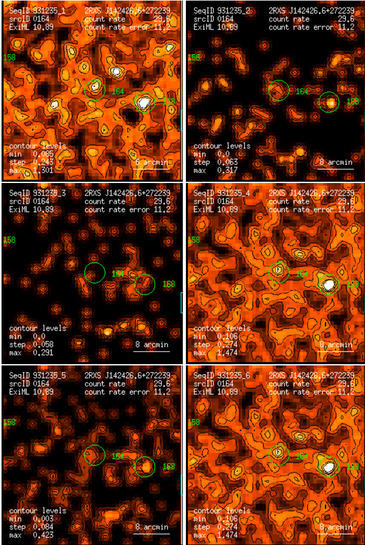
Figure 164: RASS 931235: detection 0164: band rate images, Gaussian filter: (1) PSPC channels 11 – 41, (2) 52 – 90, (3) 91 – 201, (4) 11 – 235, (5) 52 – 201, (6) 11 – 201. Broad band rates in counts/ks. Band rate contour levels in counts/ks/arcmin 2 .
