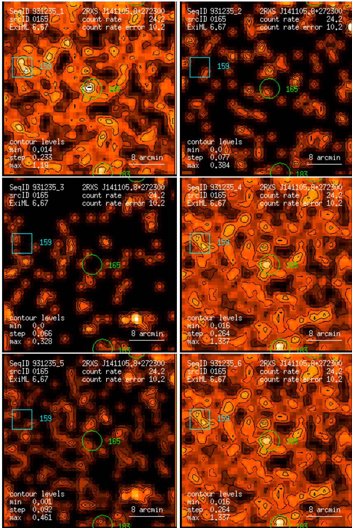
Figure 165: RASS 931235: detection 0165: band rate images, Gaussian filter: (1) PSPC channels 11 – 41, (2) 52 – 90, (3) 91 – 201, (4) 11 – 235, (5) 52 – 201, (6) 11 – 201. Broad band rates in counts/ks. Band rate contour levels in counts/ks/arcmin 2 .
