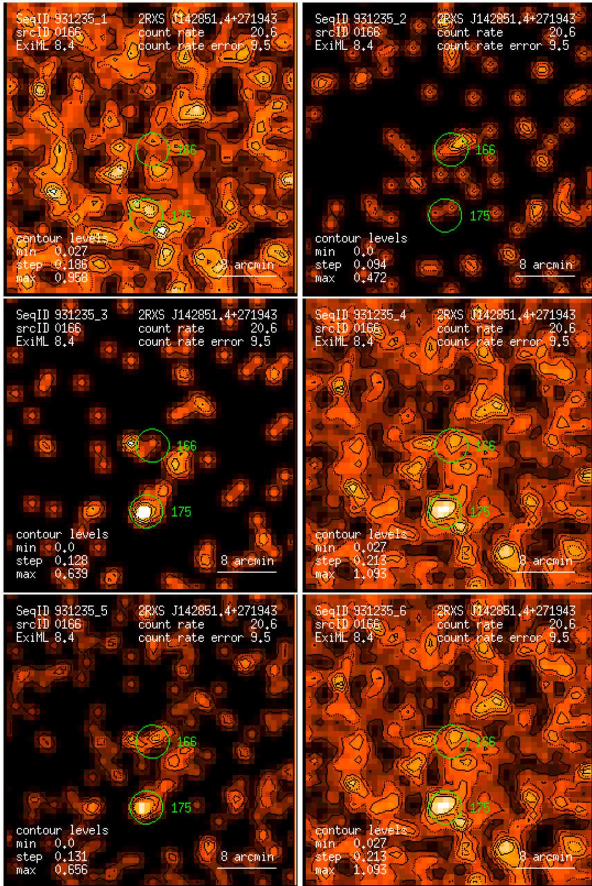
Figure 166: RASS 931235: detection 0166: band rate images, Gaussian filter: (1) PSPC channels 11 – 41, (2) 52 – 90, (3) 91 – 201, (4) 11 – 235, (5) 52 – 201, (6) 11 – 201. Broad band rates in counts/ks. Band rate contour levels in counts/ks/arcmin 2 .
