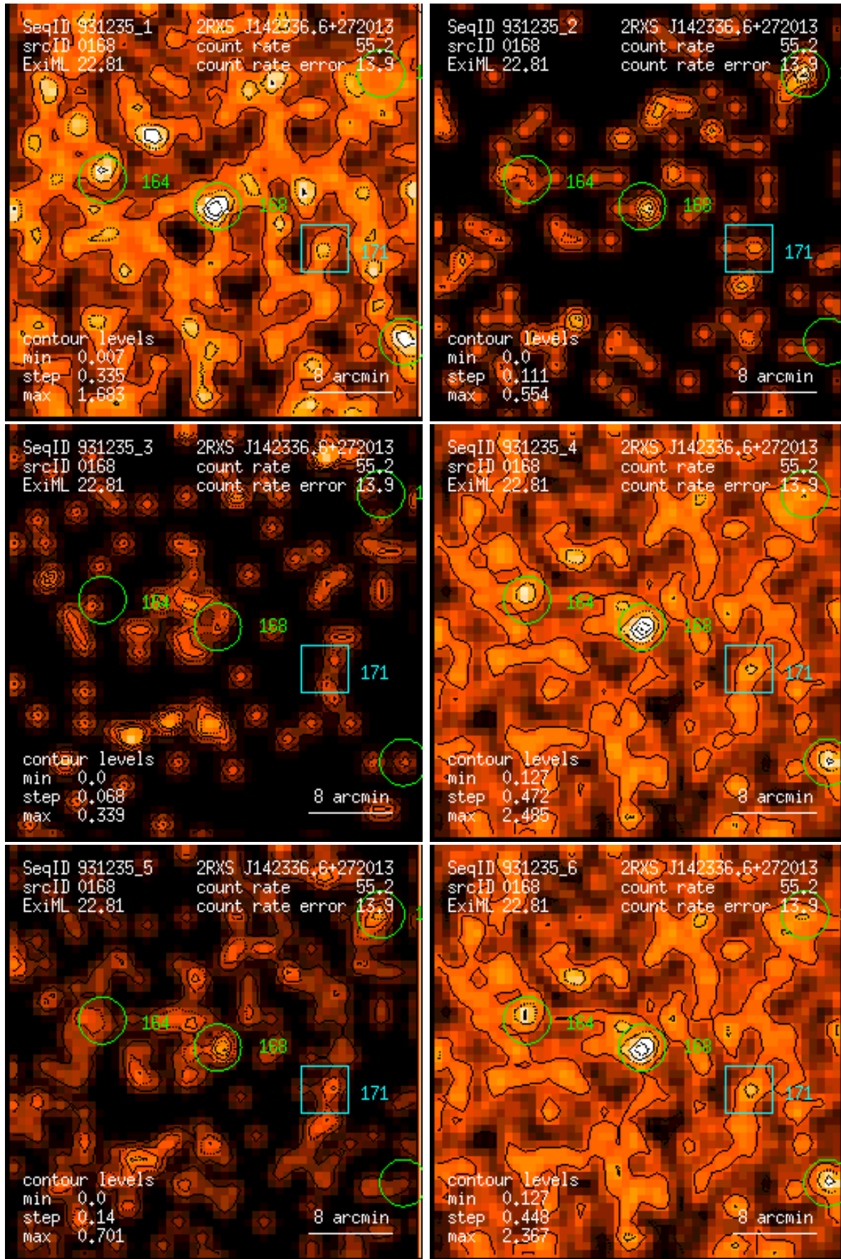
Figure 168: RASS 931235: detection 0168: band rate images, Gaussian filter: (1) PSPC channels 11 – 41, (2) 52 – 90, (3) 91 – 201, (4) 11 – 235, (5) 52 – 201, (6) 11 – 201. Broad band rates in counts/ks. Band rate contour levels in counts/ks/arcmin 2 .
