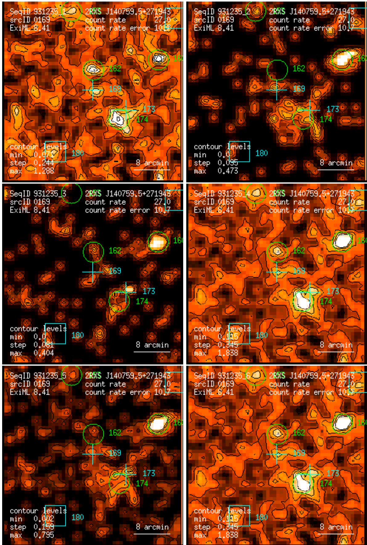
Figure 169: RASS 931235: detection 0169: band rate images, Gaussian filter: (1) PSPC channels 11 – 41, (2) 52 – 90, (3) 91 – 201, (4) 11 – 235, (5) 52 – 201, (6) 11 – 201. Broad band rates in counts/ks. Band rate contour levels in counts/ks/arcmin 2 .
