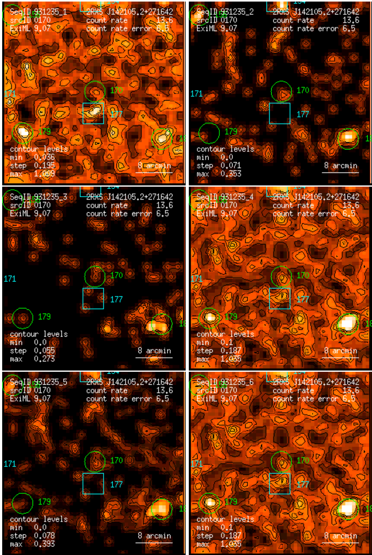
Figure 170: RASS 931235: detection 0170: band rate images, Gaussian filter: (1) PSPC channels 11 – 41, (2) 52 – 90, (3) 91 – 201, (4) 11 – 235, (5) 52 – 201, (6) 11 – 201. Broad band rates in counts/ks. Band rate contour levels in counts/ks/arcmin 2 .
