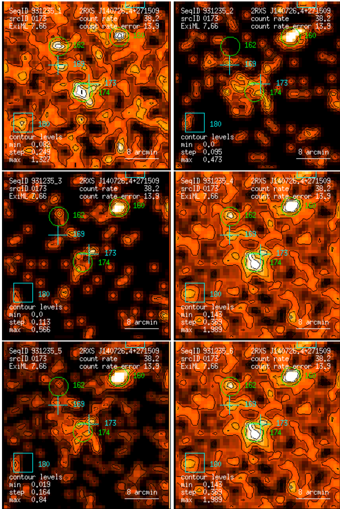
Figure 173: RASS 931235: detection 0173: band rate images, Gaussian filter: (1) PSPC channels 11 – 41, (2) 52 – 90, (3) 91 – 201, (4) 11 – 235, (5) 52 – 201, (6) 11 – 201. Broad band rates in counts/ks. Band rate contour levels in counts/ks/arcmin 2 .
