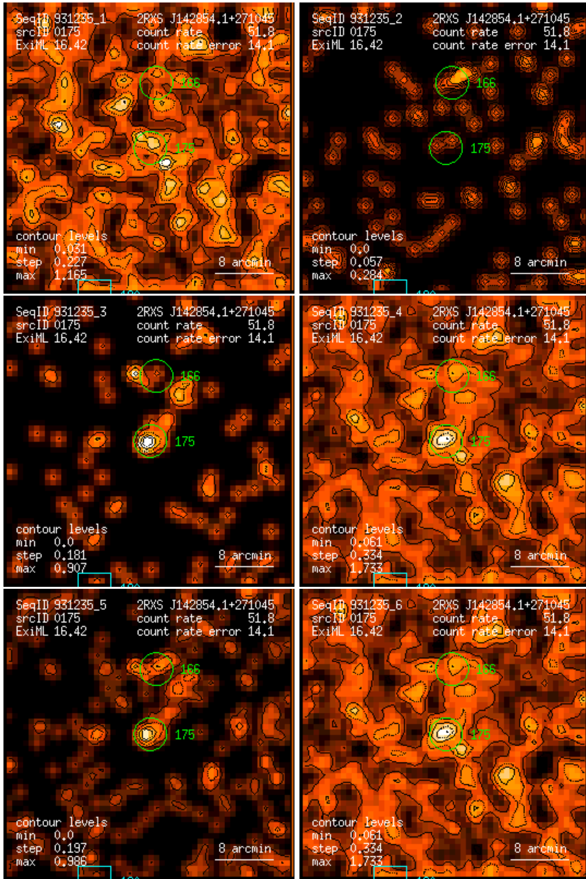
Figure 175: RASS 931235: detection 0175: band rate images, Gaussian filter: (1) PSPC channels 11 – 41, (2) 52 – 90, (3) 91 – 201, (4) 11 – 235, (5) 52 – 201, (6) 11 – 201. Broad band rates in counts/ks. Band rate contour levels in counts/ks/arcmin 2 .
