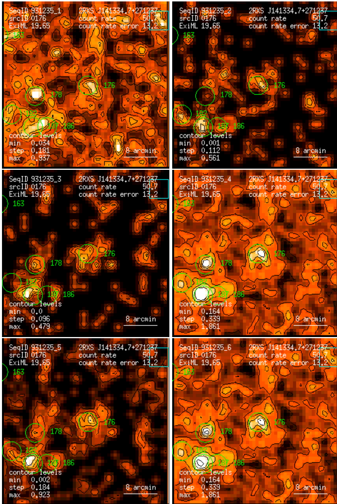
Figure 176: RASS 931235: detection 0176: band rate images, Gaussian filter: (1) PSPC channels 11 – 41, (2) 52 – 90, (3) 91 – 201, (4) 11 – 235, (5) 52 – 201, (6) 11 – 201. Broad band rates in counts/ks. Band rate contour levels in counts/ks/arcmin 2 .
