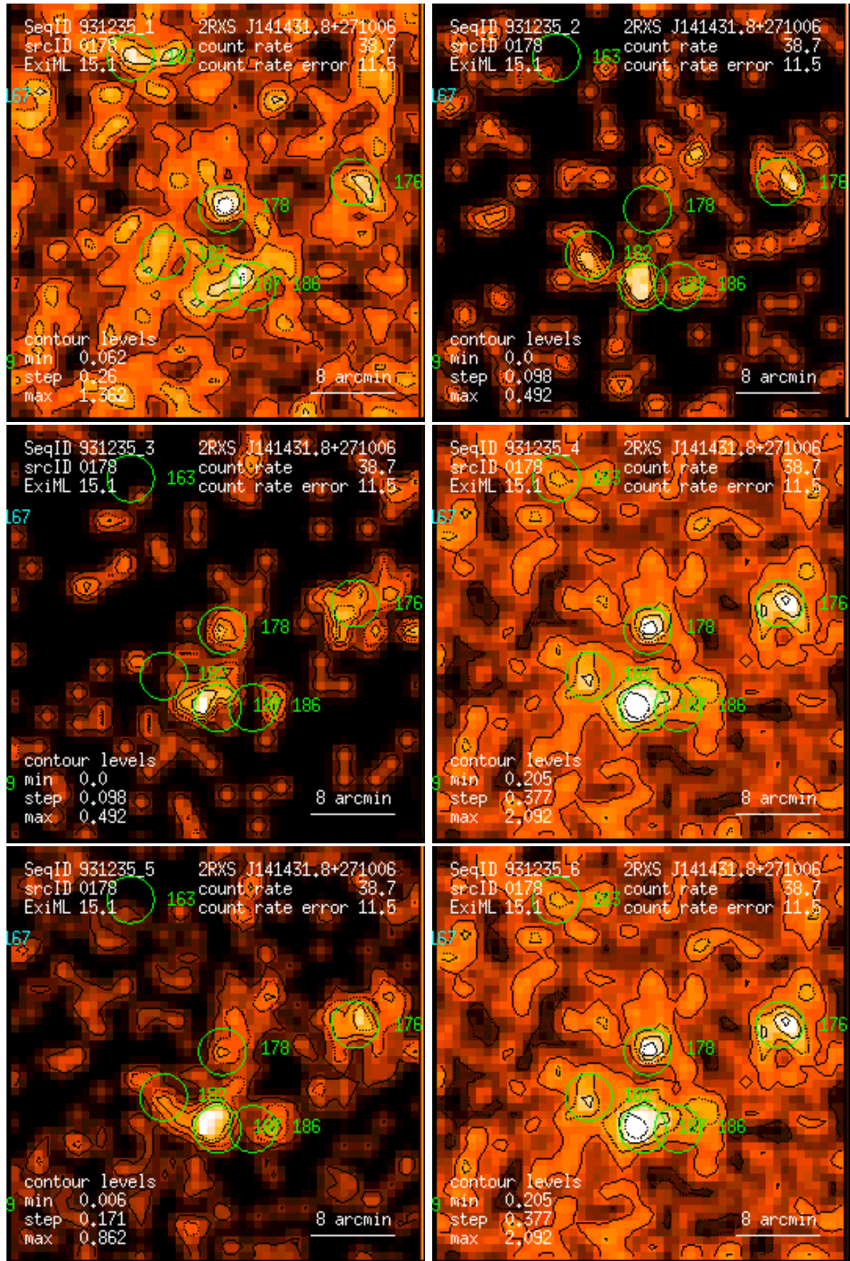
Figure 178: RASS 931235: detection 0178: band rate images, Gaussian filter: (1) PSPC channels 11 – 41, (2) 52 – 90, (3) 91 – 201, (4) 11 – 235, (5) 52 – 201, (6) 11 – 201. Broad band rates in counts/ks. Band rate contour levels in counts/ks/arcmin 2 .
