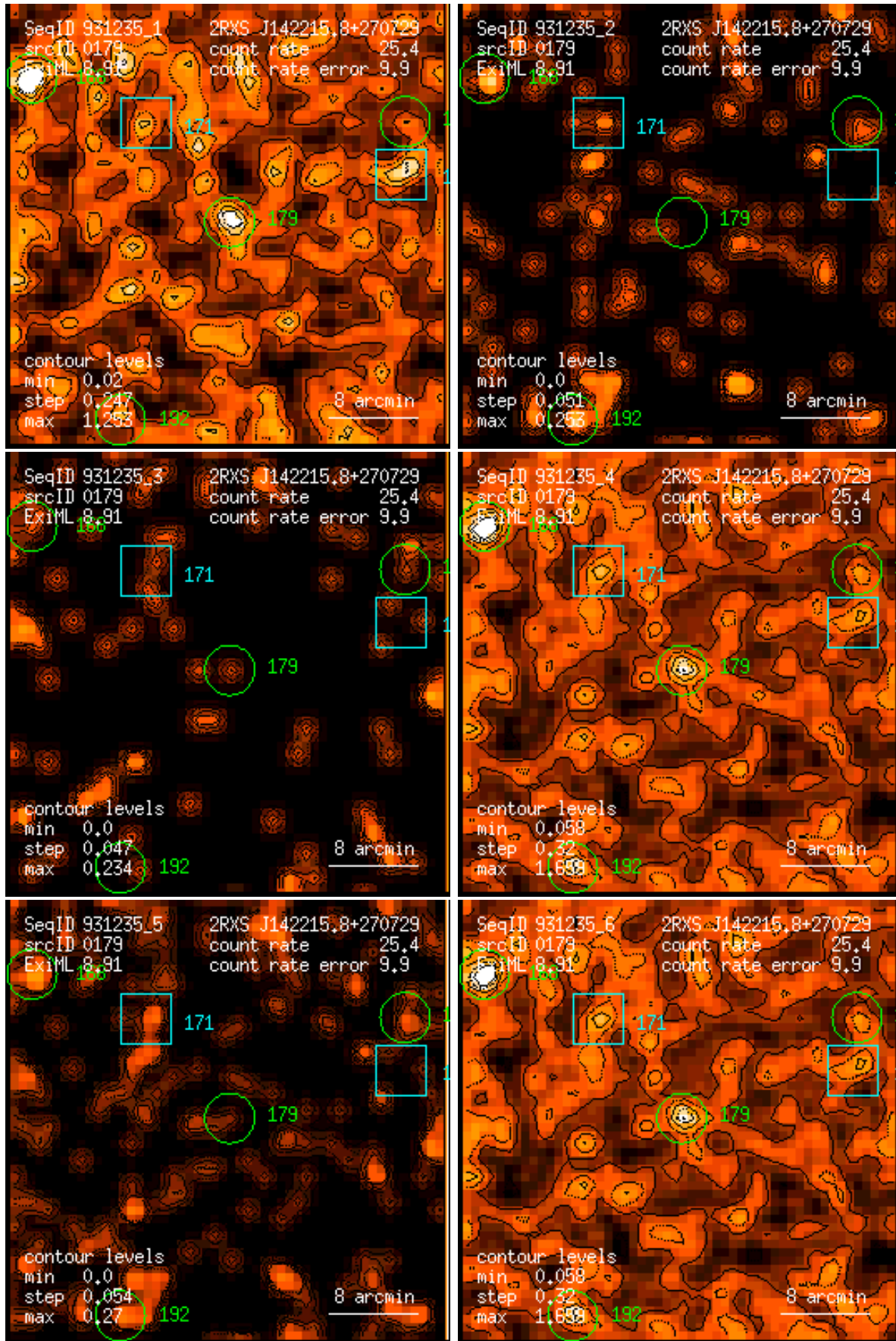
Figure 179: RASS 931235: detection 0179: band rate images, Gaussian filter: (1) PSPC channels 11 – 41, (2) 52 – 90, (3) 91 – 201, (4) 11 – 235, (5) 52 – 201, (6) 11 – 201. Broad band rates in counts/ks. Band rate contour levels in counts/ks/arcmin 2 .
