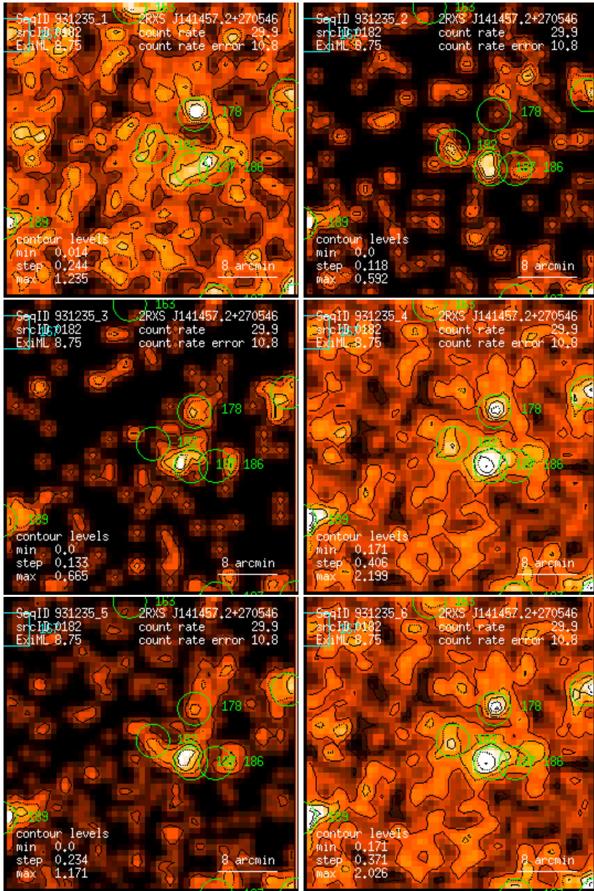
Figure 182: RASS 931235: detection 0182: band rate images, Gaussian filter: (1) PSPC channels 11 – 41, (2) 52 – 90, (3) 91 – 201, (4) 11 – 235, (5) 52 – 201, (6) 11 – 201. Broad band rates in counts/ks. Band rate contour levels in counts/ks/arcmin 2 .
