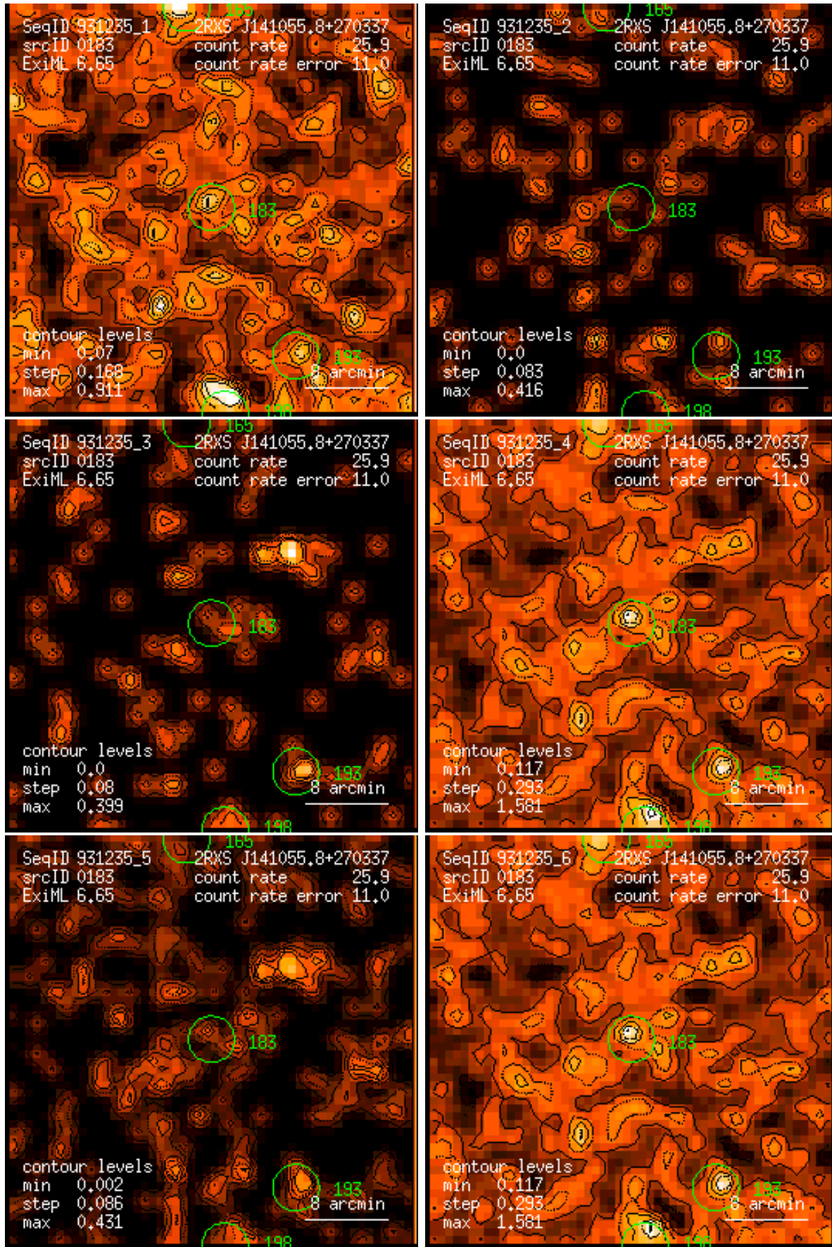
Figure 183: RASS 931235: detection 0183: band rate images, Gaussian filter: (1) PSPC channels 11 – 41, (2) 52 – 90, (3) 91 – 201, (4) 11 – 235, (5) 52 – 201, (6) 11 – 201. Broad band rates in counts/ks. Band rate contour levels in counts/ks/arcmin 2 .
