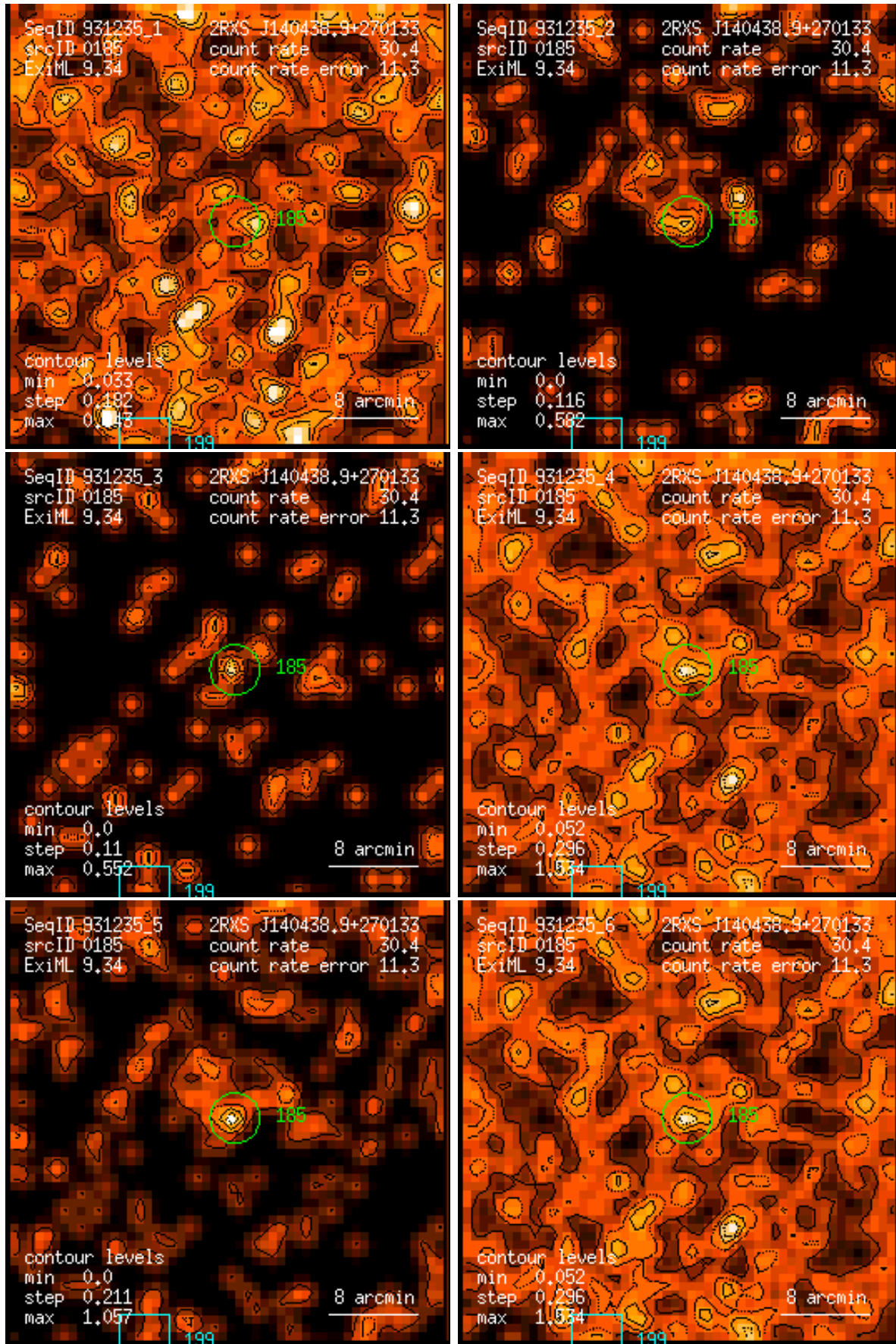
Figure 185: RASS 931235: detection 0185: band rate images, Gaussian filter: (1) PSPC channels 11 – 41, (2) 52 – 90, (3) 91 – 201, (4) 11 – 235, (5) 52 – 201, (6) 11 – 201. Broad band rates in counts/ks. Band rate contour levels in counts/ks/arcmin 2 .
