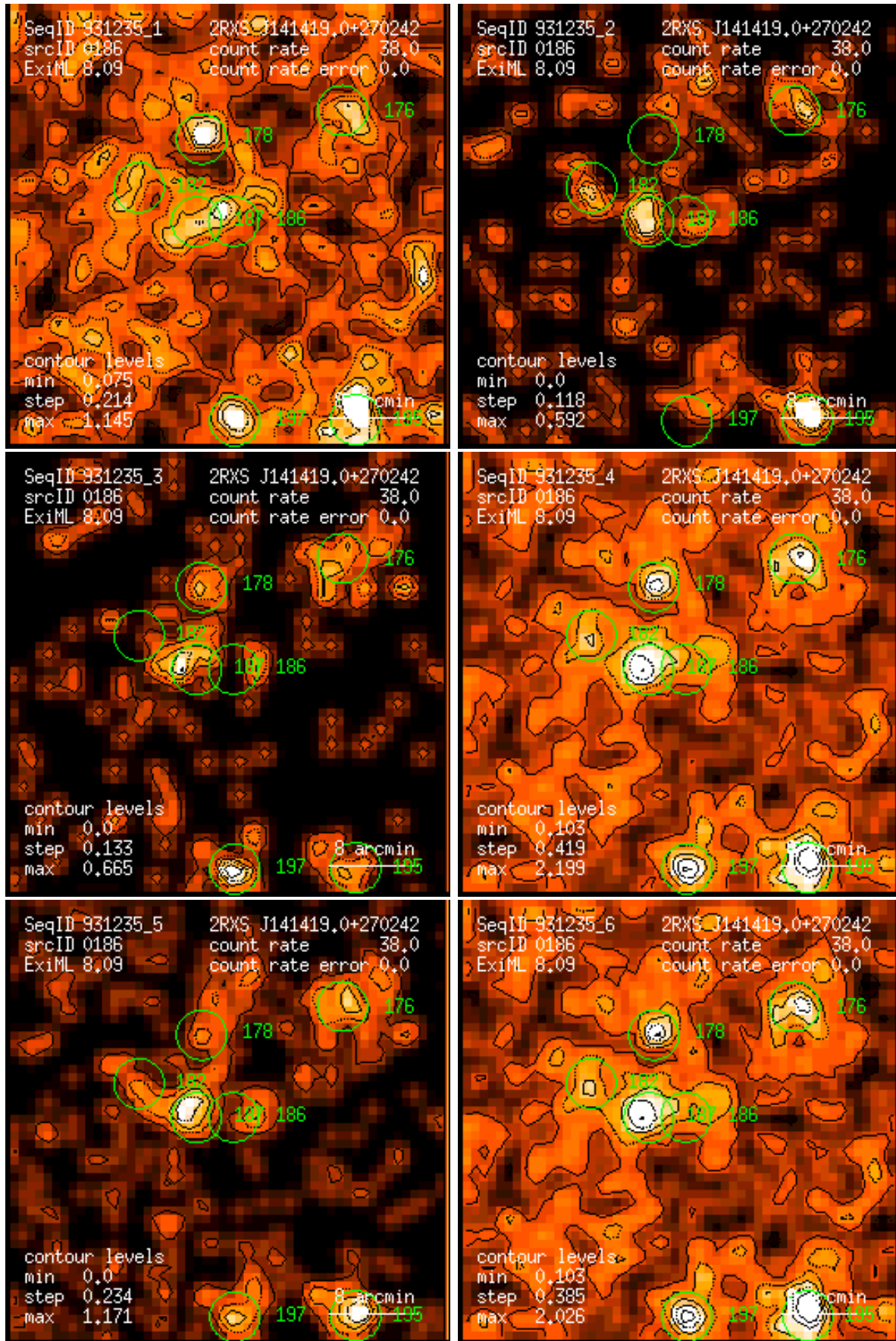
Figure 186: RASS 931235: detection 0186: band rate images, Gaussian filter: (1) PSPC channels 11 – 41, (2) 52 – 90, (3) 91 – 201, (4) 11 – 235, (5) 52 – 201, (6) 11 – 201. Broad band rates in counts/ks. Band rate contour levels in counts/ks/arcmin 2 .
