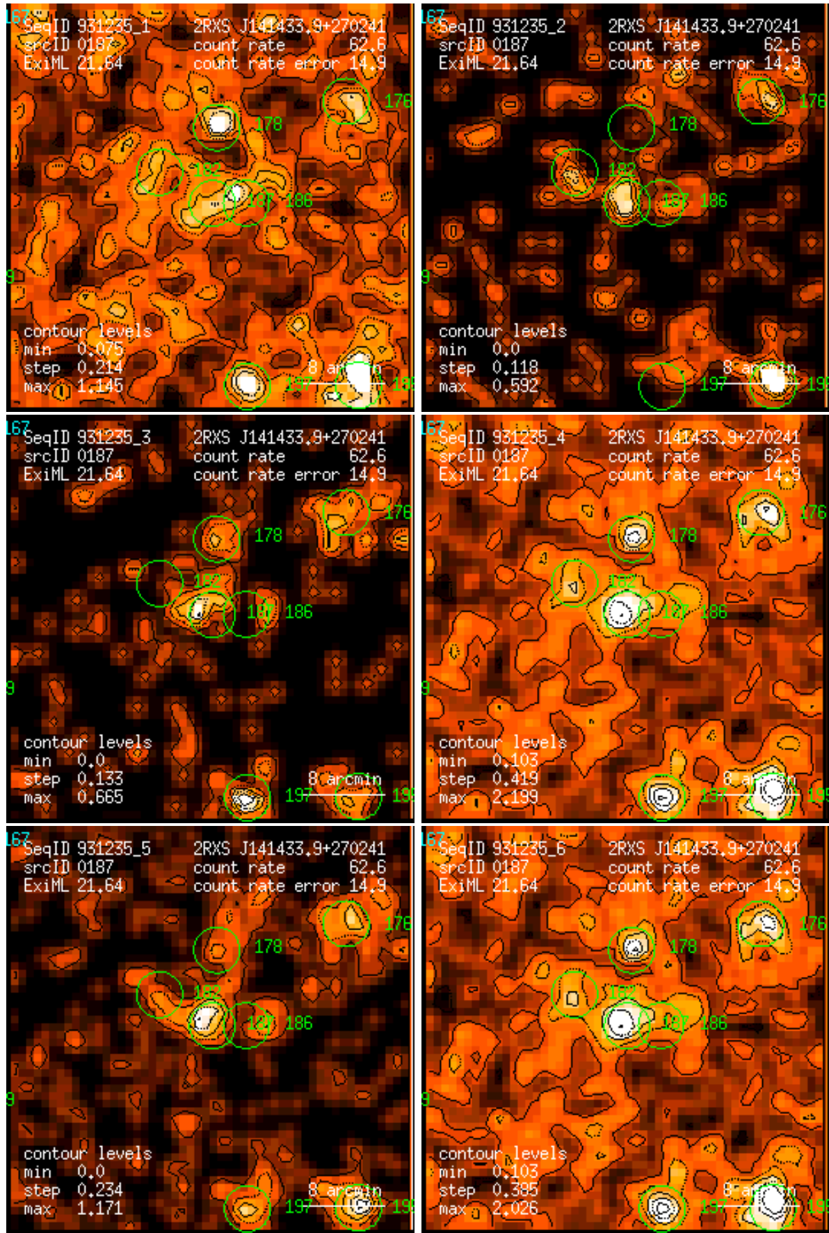
Figure 187: RASS 931235: detection 0187: band rate images, Gaussian filter: (1) PSPC channels 11 – 41, (2) 52 – 90, (3) 91 – 201, (4) 11 – 235, (5) 52 – 201, (6) 11 – 201. Broad band rates in counts/ks. Band rate contour levels in counts/ks/arcmin 2 .
