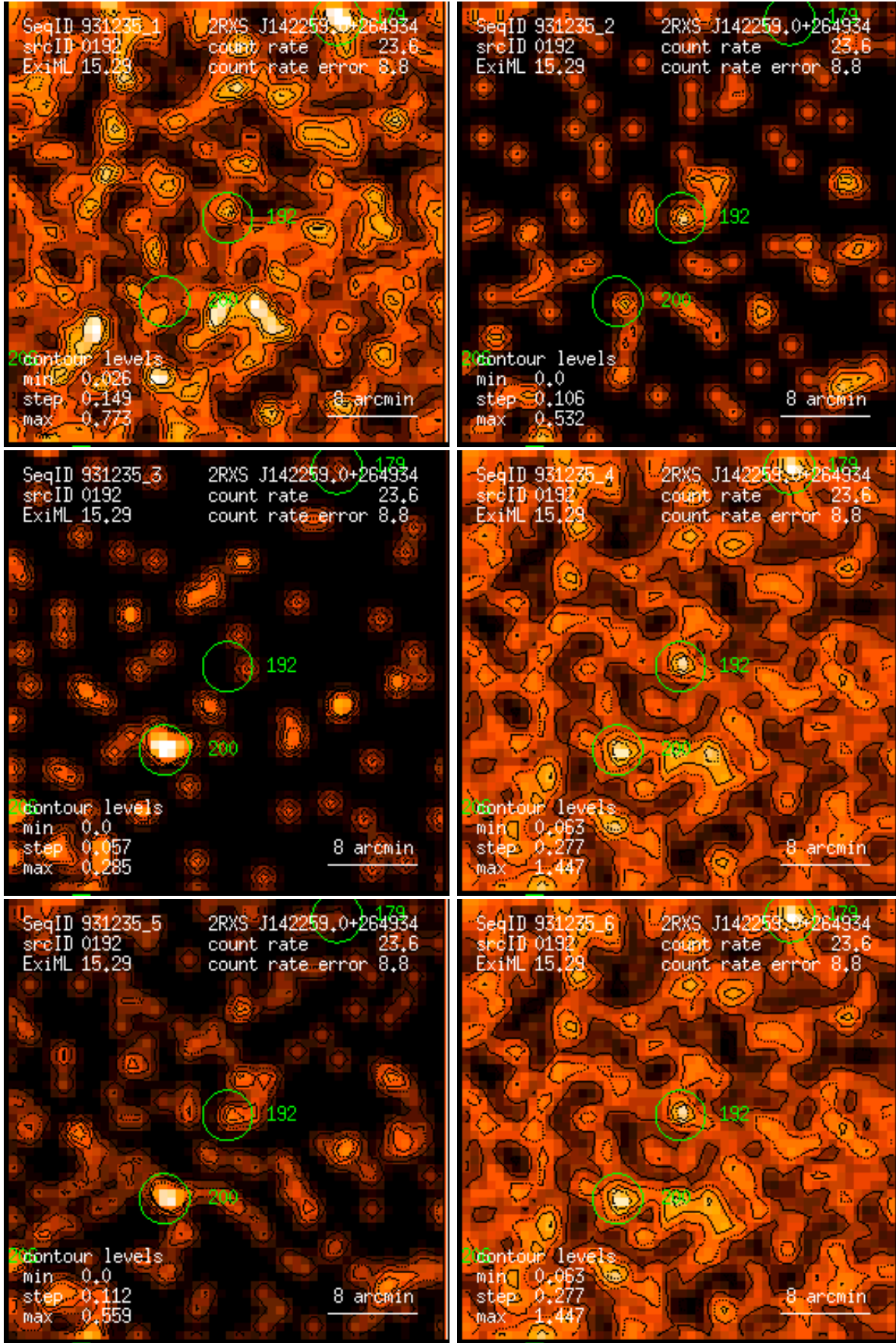
Figure 192: RASS 931235: detection 0192: band rate images, Gaussian filter: (1) PSPC channels 11 – 41, (2) 52 – 90, (3) 91 – 201, (4) 11 – 235, (5) 52 – 201, (6) 11 – 201. Broad band rates in counts/ks. Band rate contour levels in counts/ks/arcmin 2 .
