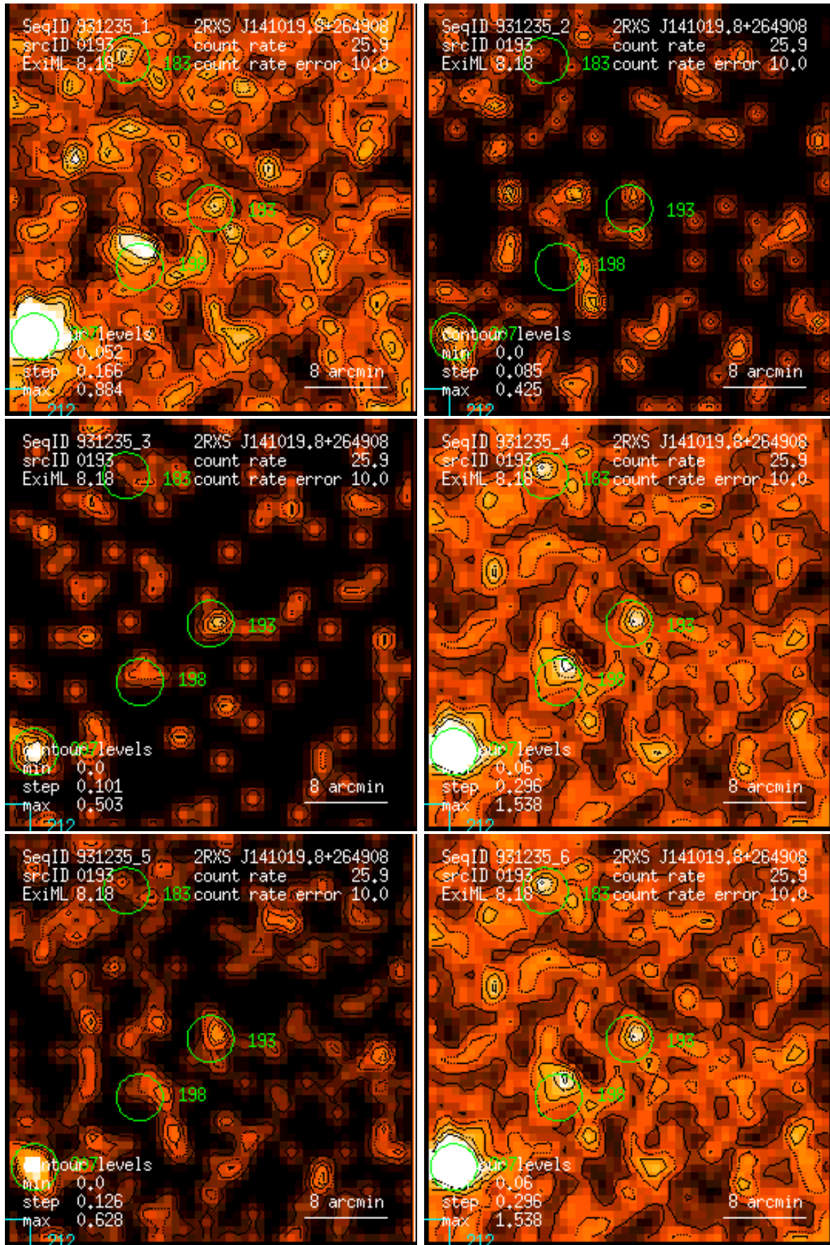
Figure 193: RASS 931235: detection 0193: band rate images, Gaussian filter: (1) PSPC channels 11 – 41, (2) 52 – 90, (3) 91 – 201, (4) 11 – 235, (5) 52 – 201, (6) 11 – 201. Broad band rates in counts/ks. Band rate contour levels in counts/ks/arcmin 2 .
