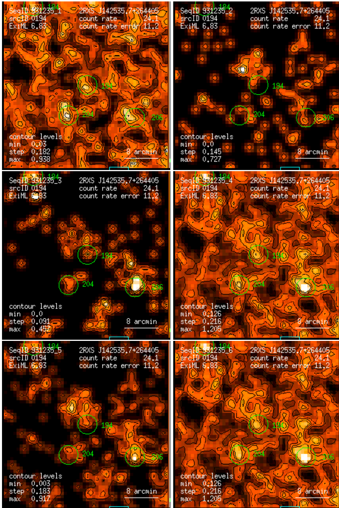
Figure 194: RASS 931235: detection 0194: band rate images, Gaussian filter: (1) PSPC channels 11 – 41, (2) 52 – 90, (3) 91 – 201, (4) 11 – 235, (5) 52 – 201, (6) 11 – 201. Broad band rates in counts/ks. Band rate contour levels in counts/ks/arcmin 2 .
