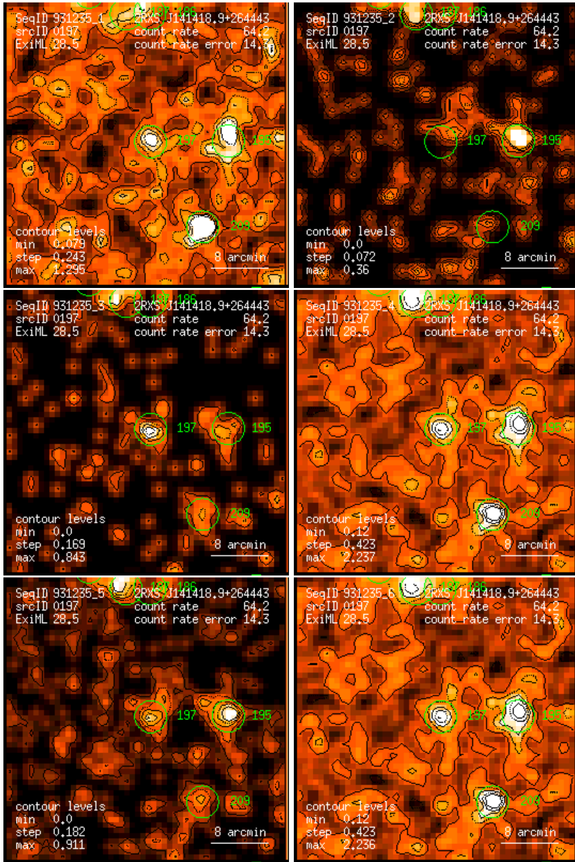
Figure 197: RASS 931235: detection 0197: band rate images, Gaussian filter: (1) PSPC channels 11 – 41, (2) 52 – 90, (3) 91 – 201, (4) 11 – 235, (5) 52 – 201, (6) 11 – 201. Broad band rates in counts/ks. Band rate contour levels in counts/ks/arcmin 2 .
