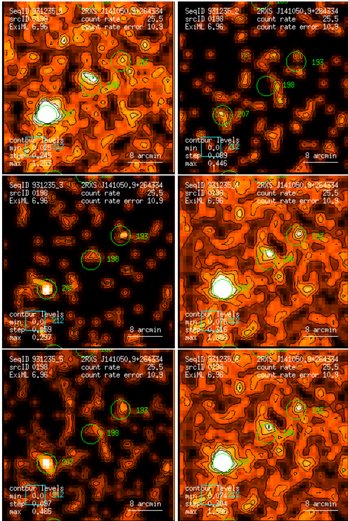
Figure 198: RASS 931235: detection 0198: band rate images, Gaussian filter: (1) PSPC channels 11 – 41, (2) 52 – 90, (3) 91 – 201, (4) 11 – 235, (5) 52 – 201, (6) 11 – 201. Broad band rates in counts/ks. Band rate contour levels in counts/ks/arcmin 2 .
