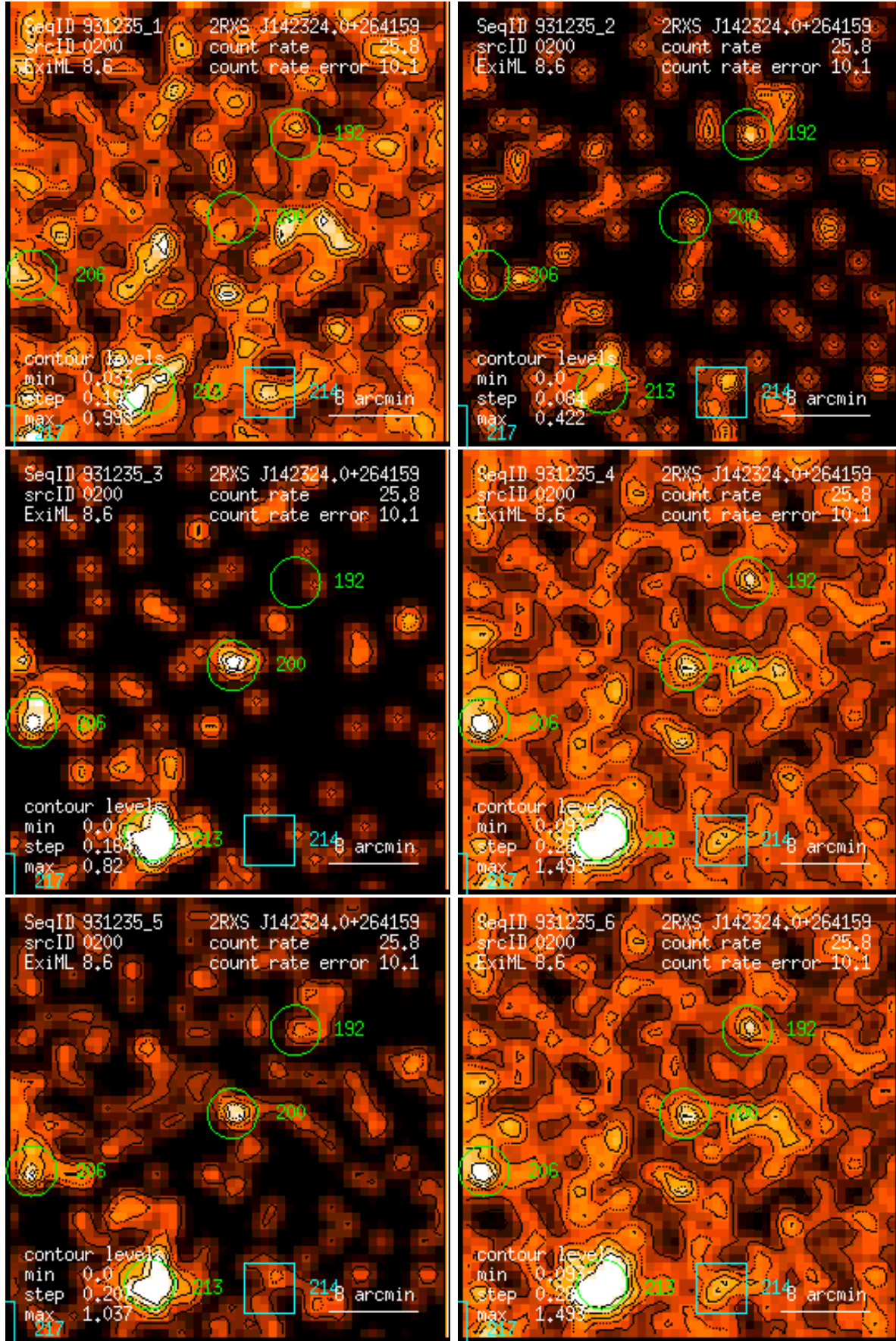
Figure 200: RASS 931235: detection 0200: band rate images, Gaussian filter: (1) PSPC channels 11 – 41, (2) 52 – 90, (3) 91 – 201, (4) 11 – 235, (5) 52 – 201, (6) 11 – 201. Broad band rates in counts/ks. Band rate contour levels in counts/ks/arcmin 2 .
