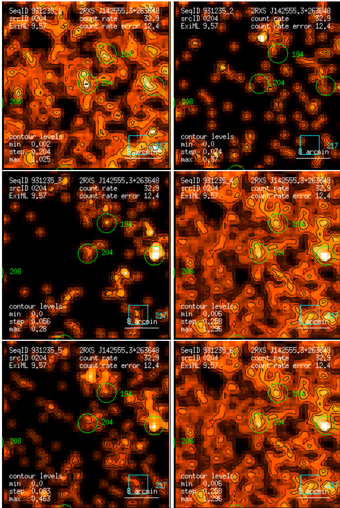
Figure 204: RASS 931235: detection 0204: band rate images, Gaussian filter: (1) PSPC channels 11 – 41, (2) 52 – 90, (3) 91 – 201, (4) 11 – 235, (5) 52 – 201, (6) 11 – 201. Broad band rates in counts/ks. Band rate contour levels in counts/ks/arcmin 2 .
