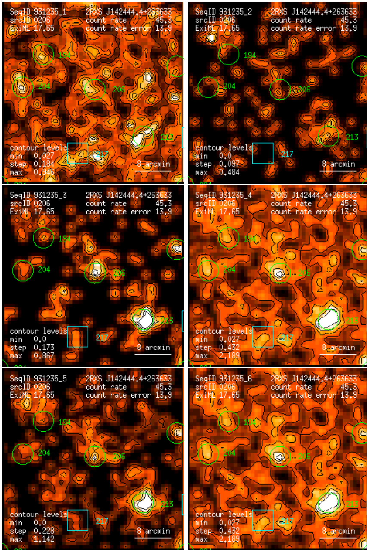
Figure 206: RASS 931235: detection 0206: band rate images, Gaussian filter: (1) PSPC channels 11 – 41, (2) 52 – 90, (3) 91 – 201, (4) 11 – 235, (5) 52 – 201, (6) 11 – 201. Broad band rates in counts/ks. Band rate contour levels in counts/ks/arcmin 2 .
