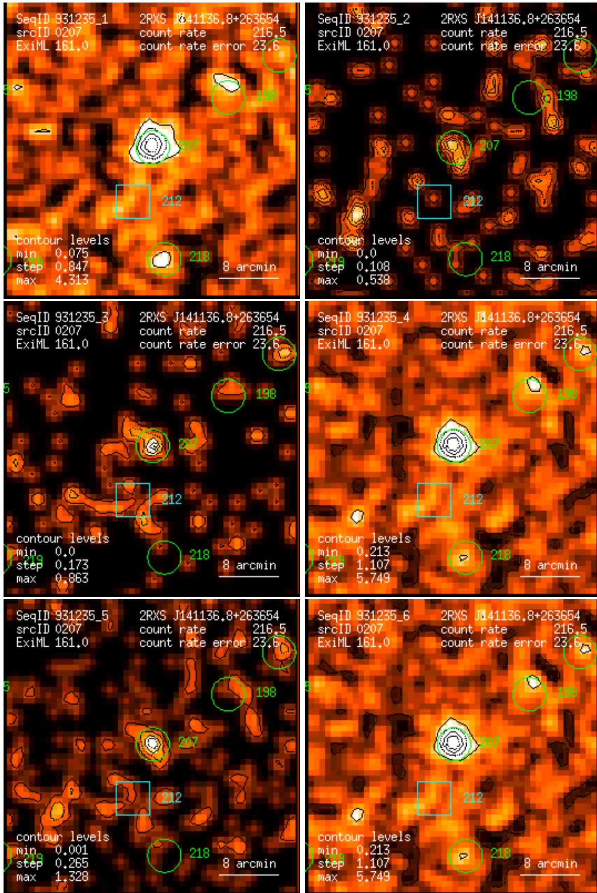
Figure 207: RASS 931235: detection 0207: band rate images, Gaussian filter: (1) PSPC channels 11 – 41, (2) 52 – 90, (3) 91 – 201, (4) 11 – 235, (5) 52 – 201, (6) 11 – 201. Broad band rates in counts/ks. Band rate contour levels in counts/ks/arcmin 2 .
