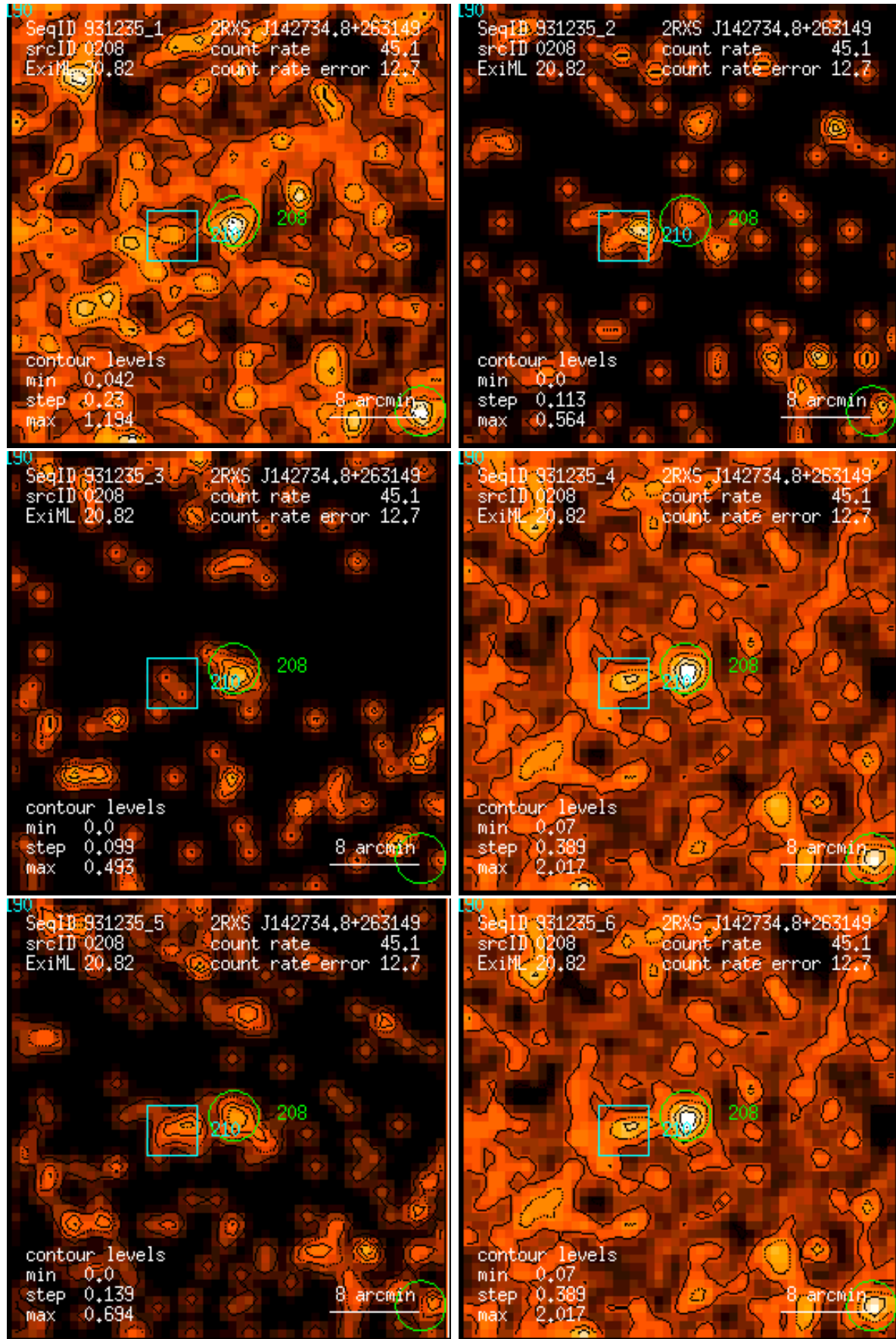
Figure 208: RASS 931235: detection 0208: band rate images, Gaussian filter: (1) PSPC channels 11 – 41, (2) 52 – 90, (3) 91 – 201, (4) 11 – 235, (5) 52 – 201, (6) 11 – 201. Broad band rates in counts/ks. Band rate contour levels in counts/ks/arcmin 2 .
