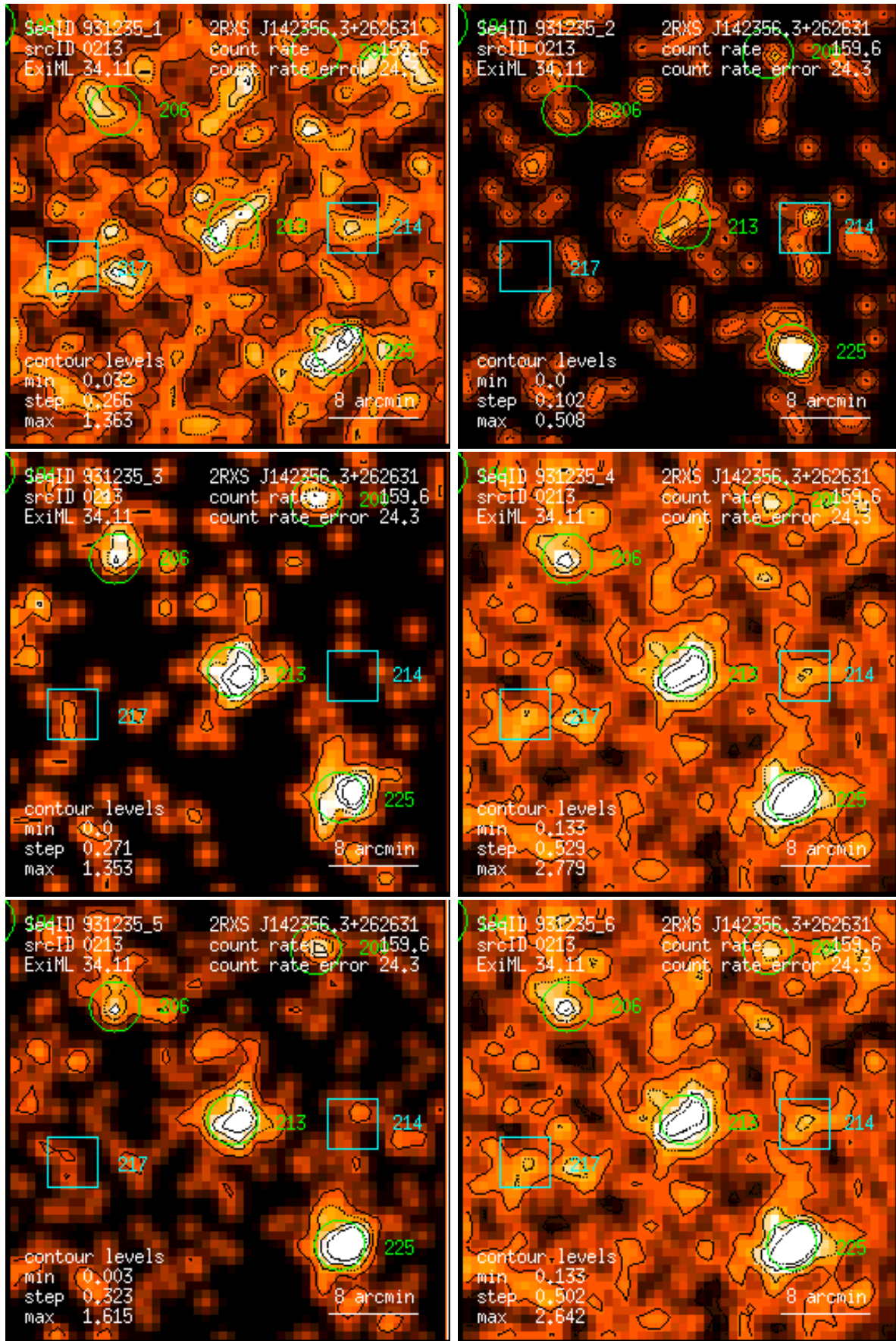
Figure 213: RASS 931235: detection 0213: band rate images, Gaussian filter: (1) PSPC channels 11 – 41, (2) 52 – 90, (3) 91 – 201, (4) 11 – 235, (5) 52 – 201, (6) 11 – 201. Broad band rates in counts/ks. Band rate contour levels in counts/ks/arcmin 2 .
