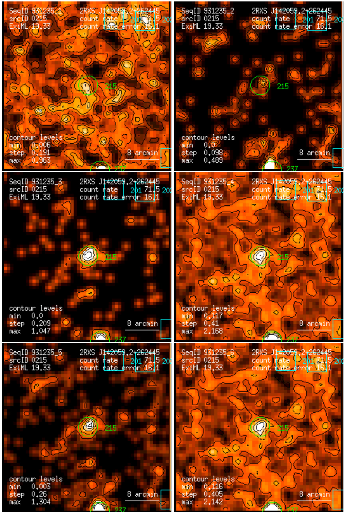
Figure 215: RASS 931235: detection 0215: band rate images, Gaussian filter: (1) PSPC channels 11 – 41, (2) 52 – 90, (3) 91 – 201, (4) 11 – 235, (5) 52 – 201, (6) 11 – 201. Broad band rates in counts/ks. Band rate contour levels in counts/ks/arcmin 2 .
