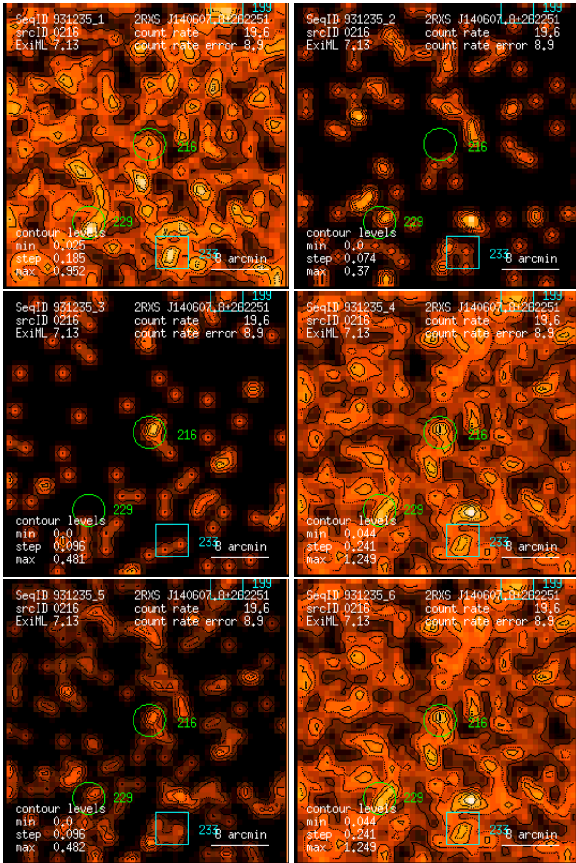
Figure 216: RASS 931235: detection 0216: band rate images, Gaussian filter: (1) PSPC channels 11 – 41, (2) 52 – 90, (3) 91 – 201, (4) 11 – 235, (5) 52 – 201, (6) 11 – 201. Broad band rates in counts/ks. Band rate contour levels in counts/ks/arcmin 2 .
