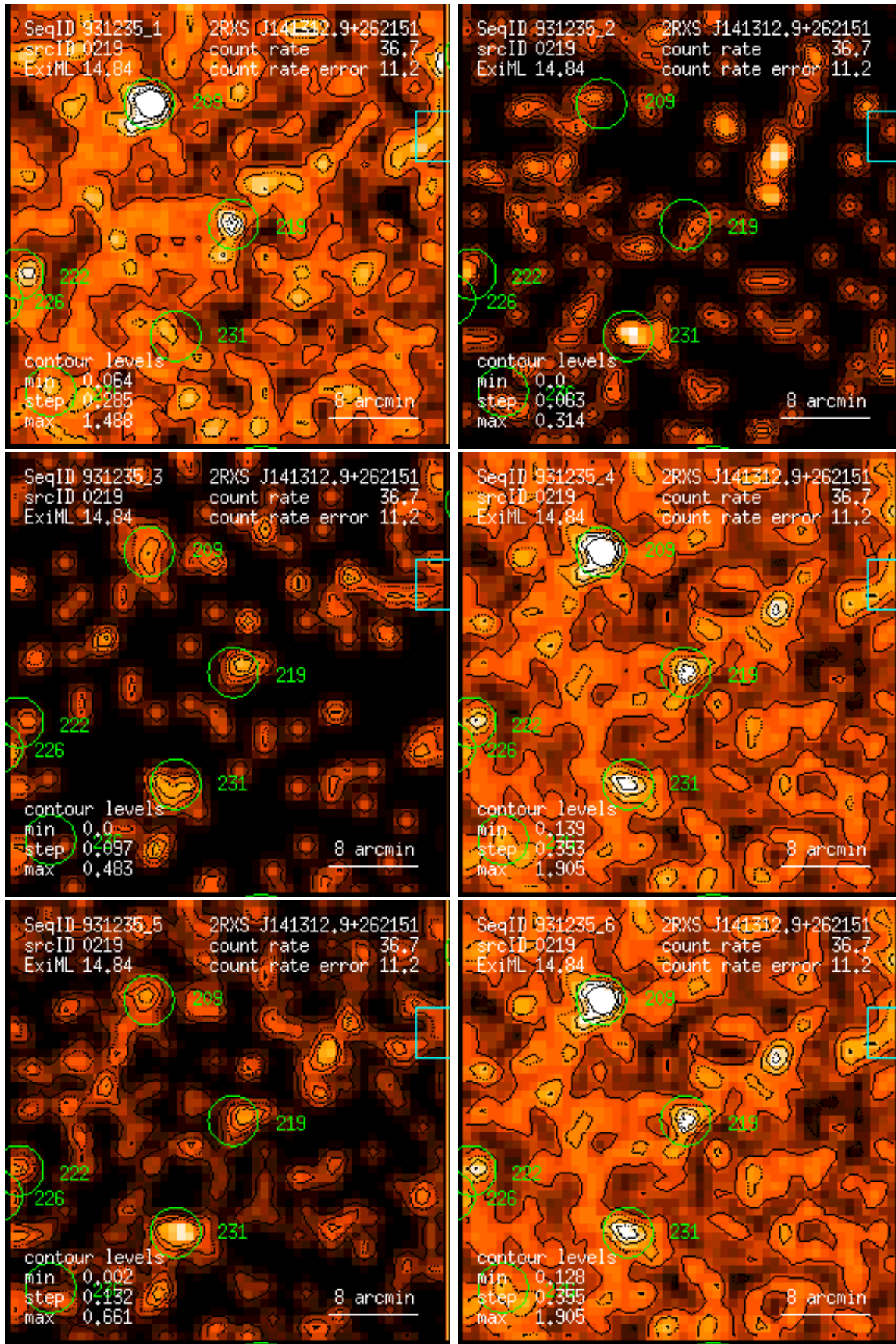
Figure 219: RASS 931235: detection 0219: band rate images, Gaussian filter: (1) PSPC channels 11 – 41, (2) 52 – 90, (3) 91 – 201, (4) 11 – 235, (5) 52 – 201, (6) 11 – 201. Broad band rates in counts/ks. Band rate contour levels in counts/ks/arcmin 2 .
